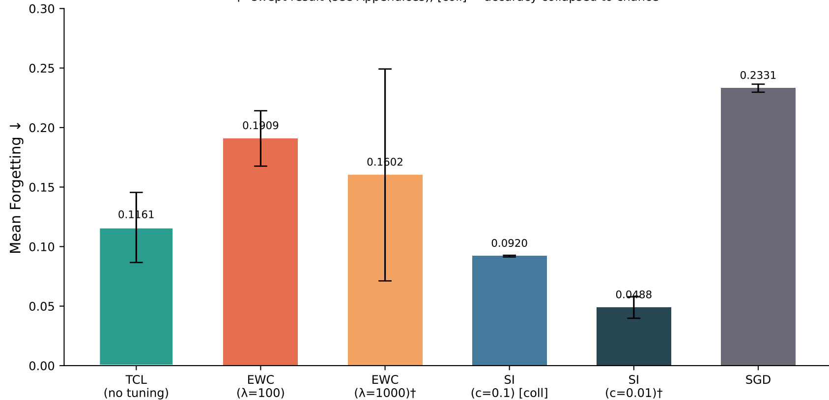
Primary baseline comparison: mean forgetting \pm std †~swept result (see Appendices); [coll] = accuracy collapsed to chance
