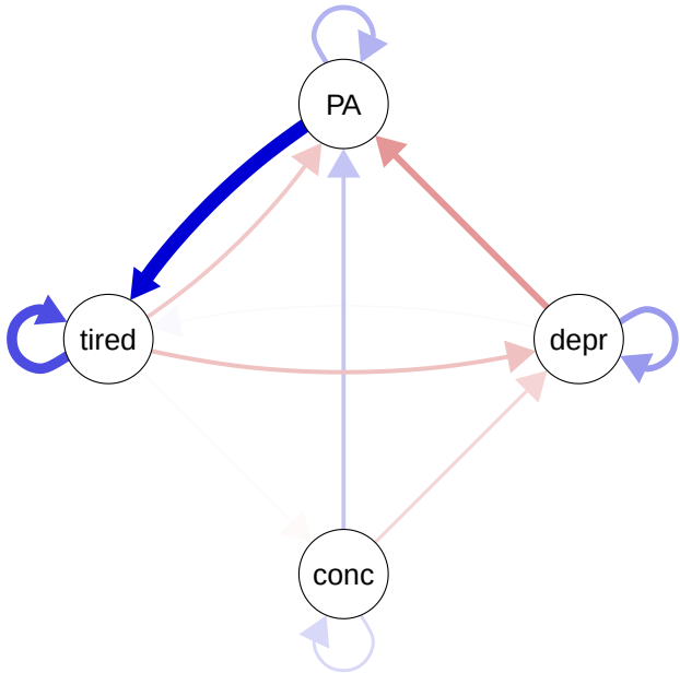
Individual B: Temporal Network
