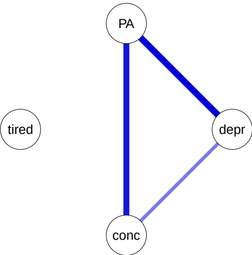
Individual A: Contemporaneous Network
