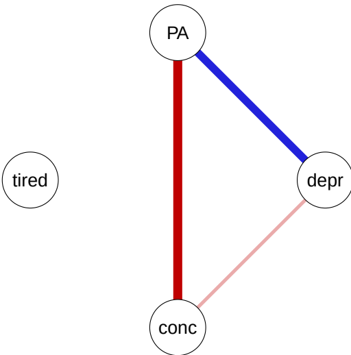
Individual B: Contemporaneous Network
