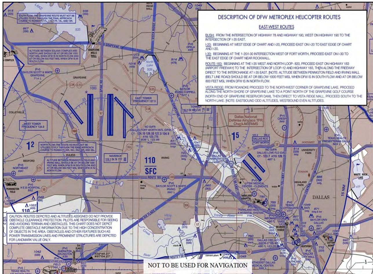
FIG 3-5-4 Helicopter Route Chart
