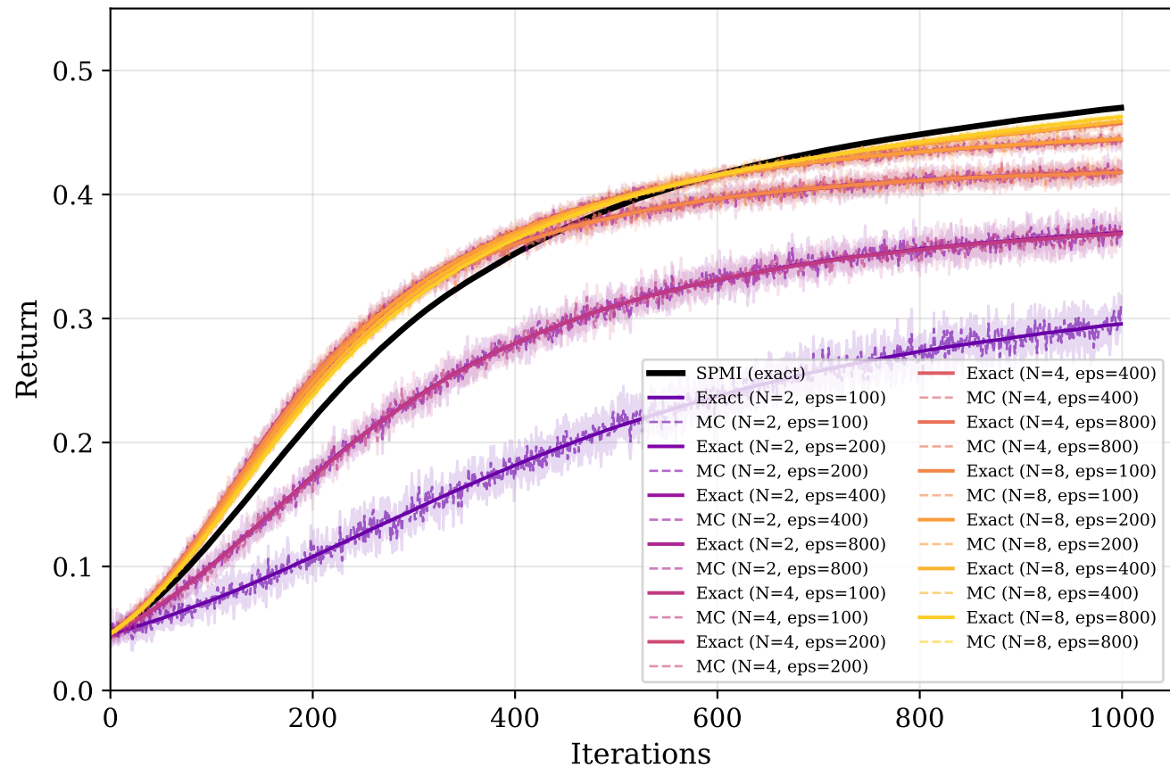
GP: MC vs Exact
