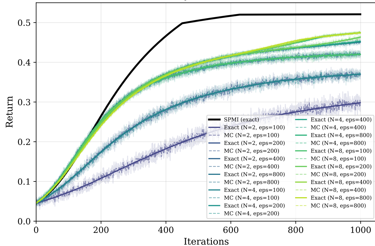
Greedy: MC vs Exact
