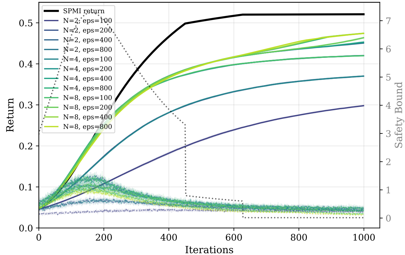
Greedy: Returns (solid) &amp; Safety Bounds (dotted)
