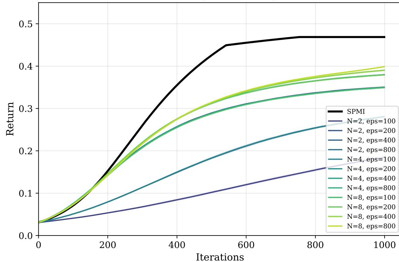
Convergence: Greedy
