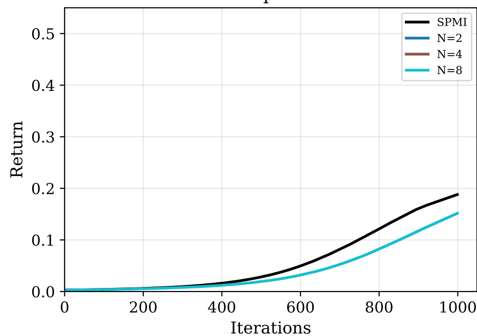
GP - eps=100
