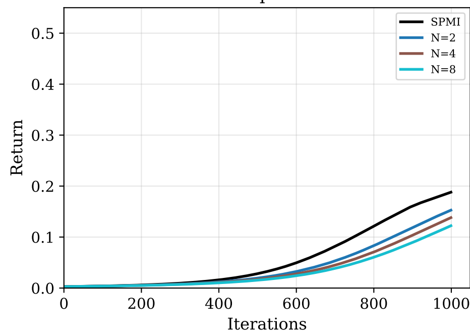
GP - eps=400
