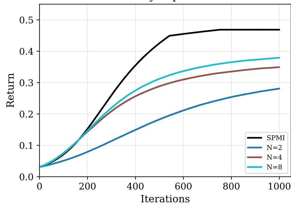
GP - eps=200
