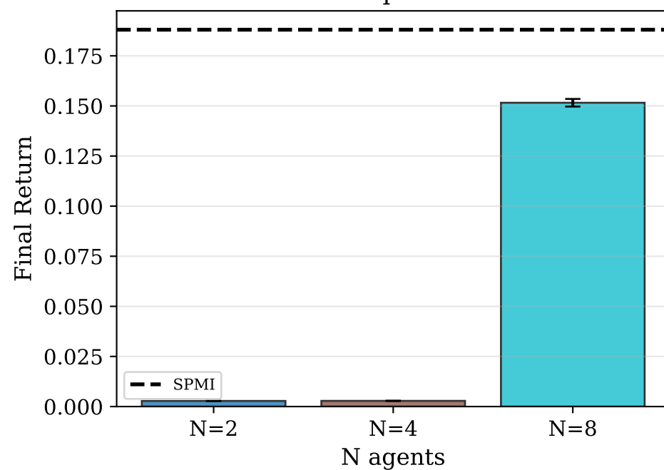
GP - eps=100
