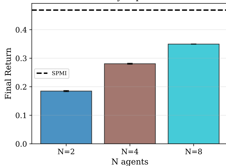
GP - eps=100
