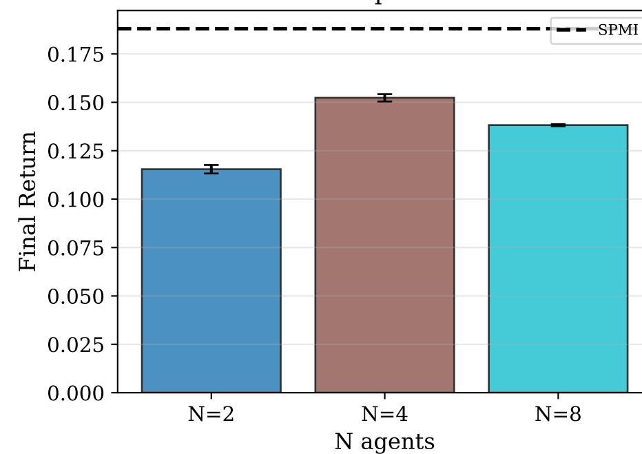
GP - eps=200
