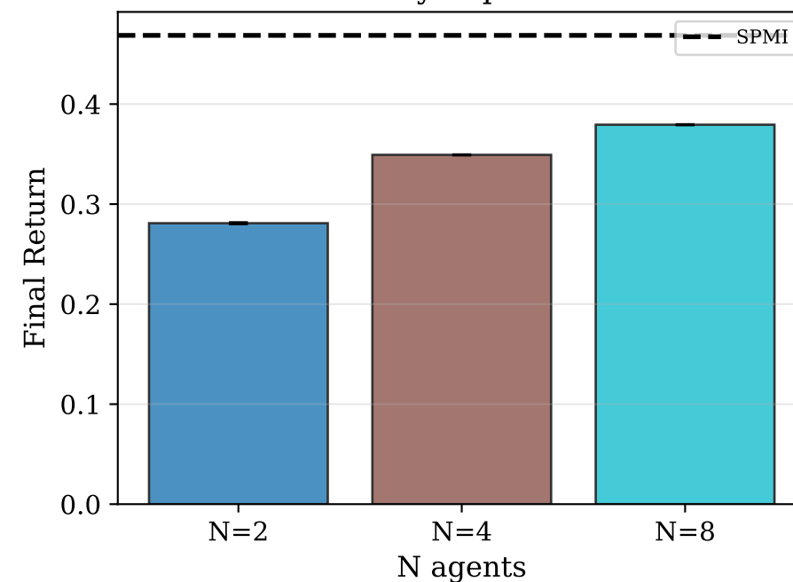
GP - eps=200
