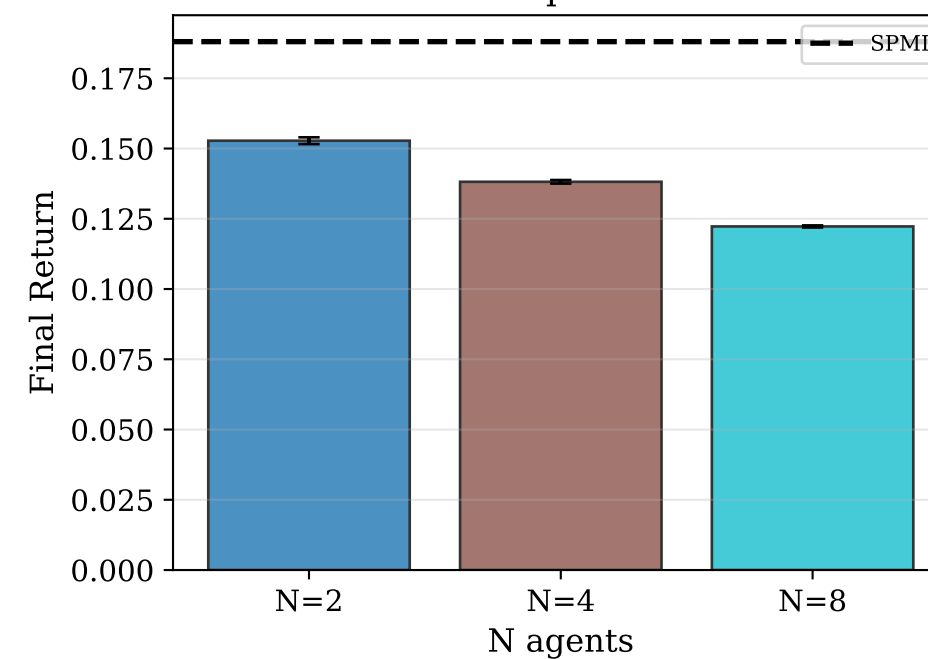
GP - eps=400
