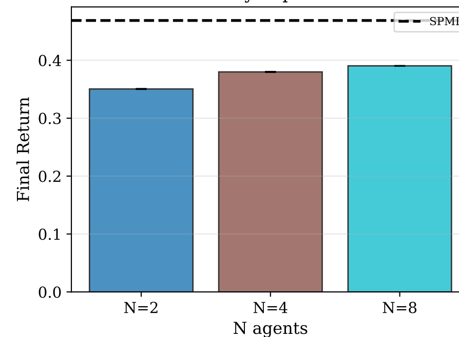
GP - eps=400
