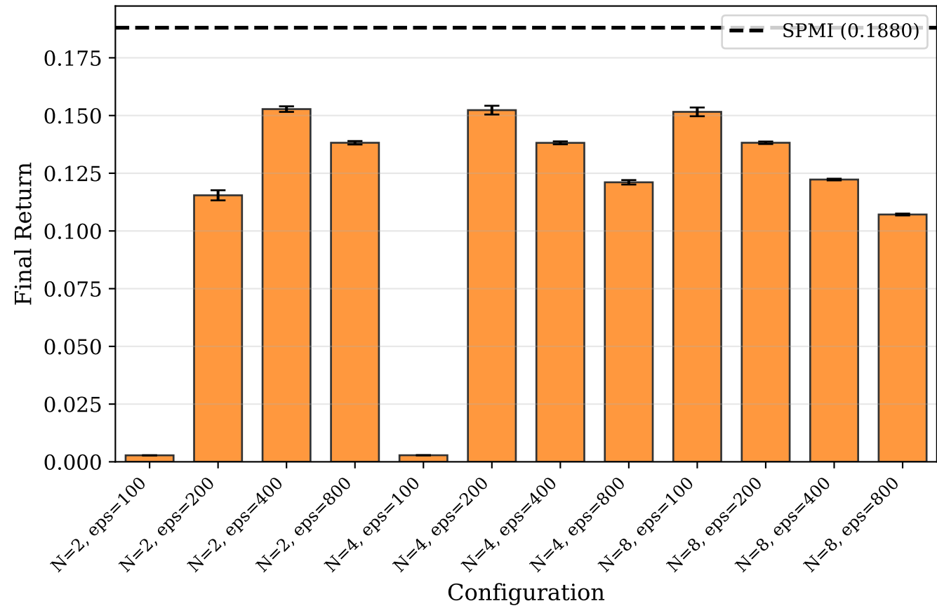
Final Performance: GP
