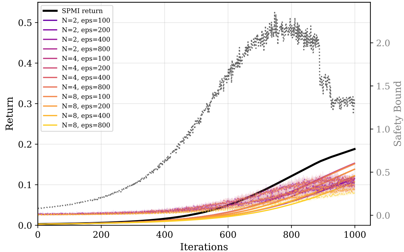
GP: Returns (solid) &amp; Safety Bounds (dotted)
