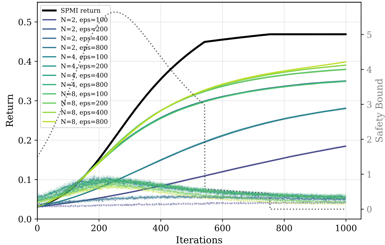
Greedy: Returns (solid) &amp; Safety Bounds (dotted)
