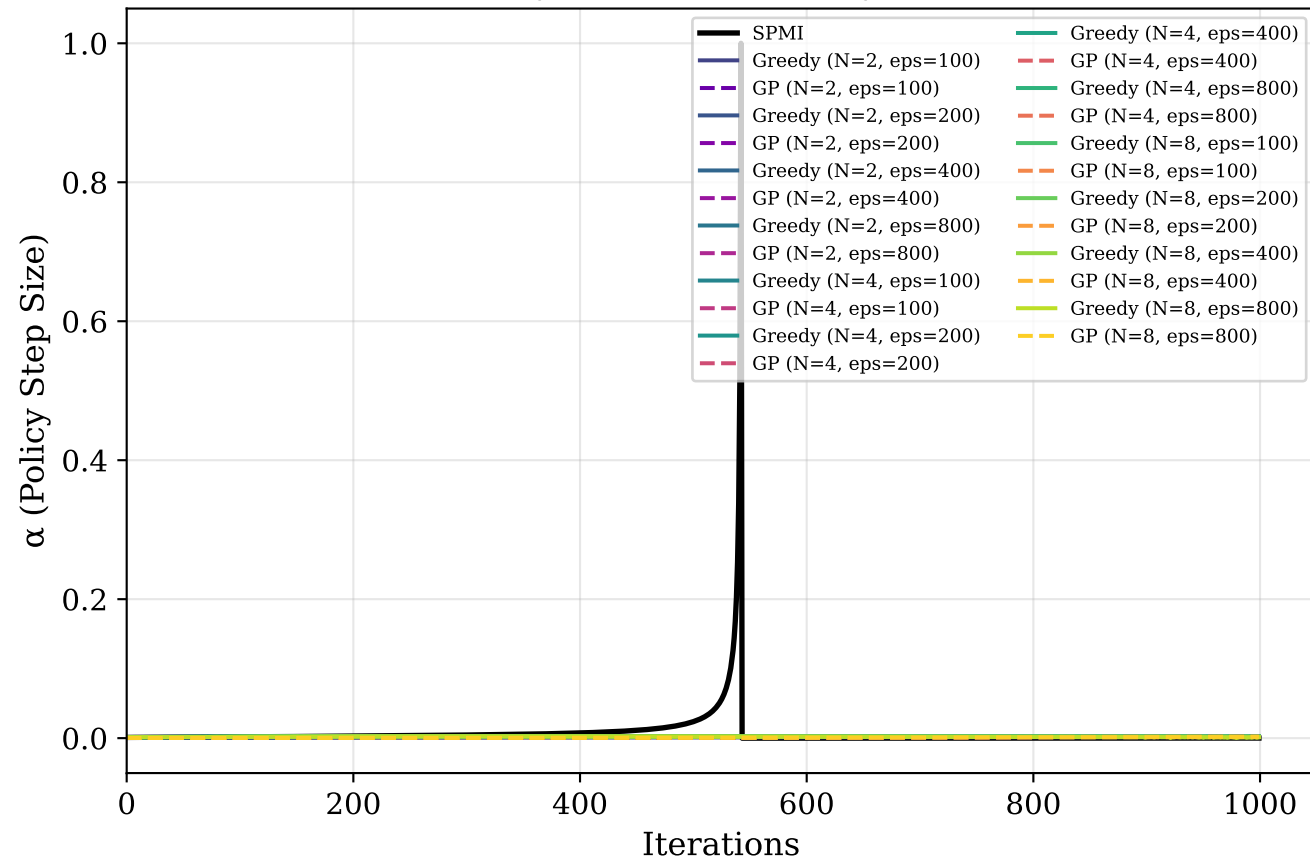
Policy Step Size: Greedy vs GP
