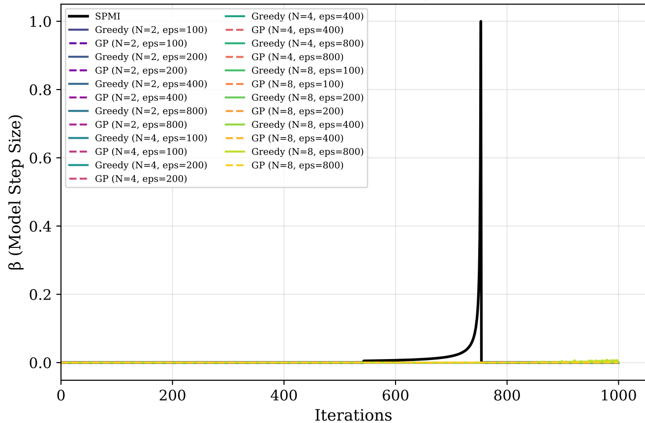
Model Step Size: Greedy vs GP
