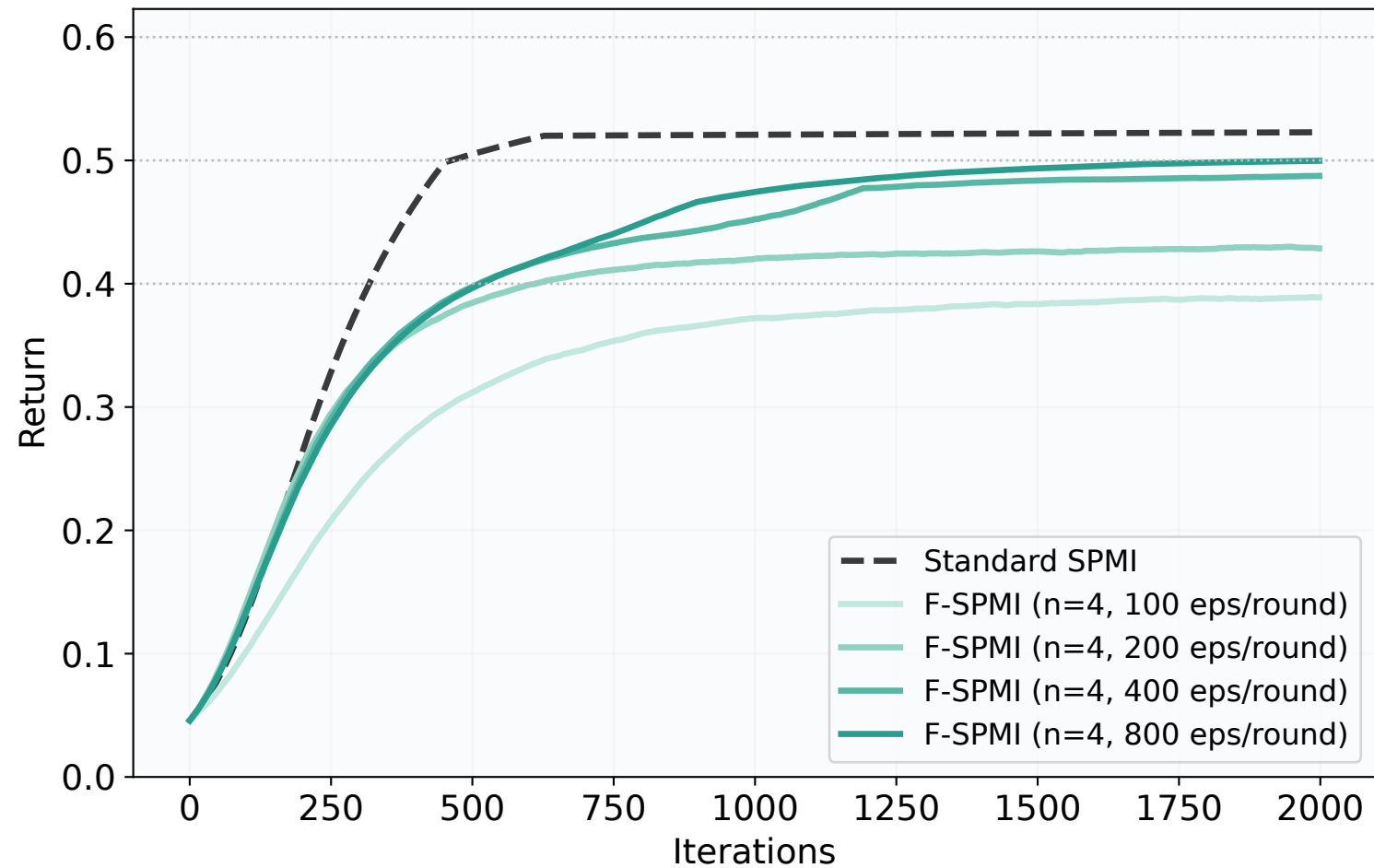
GREEDY chooser: Standard vs F-SPMI
