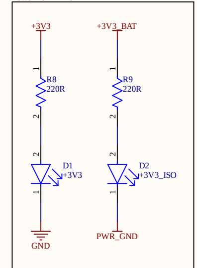
Power Rail LEDs
