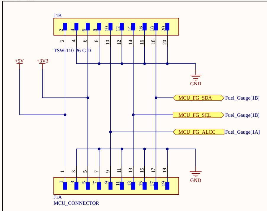
MCU Connector
