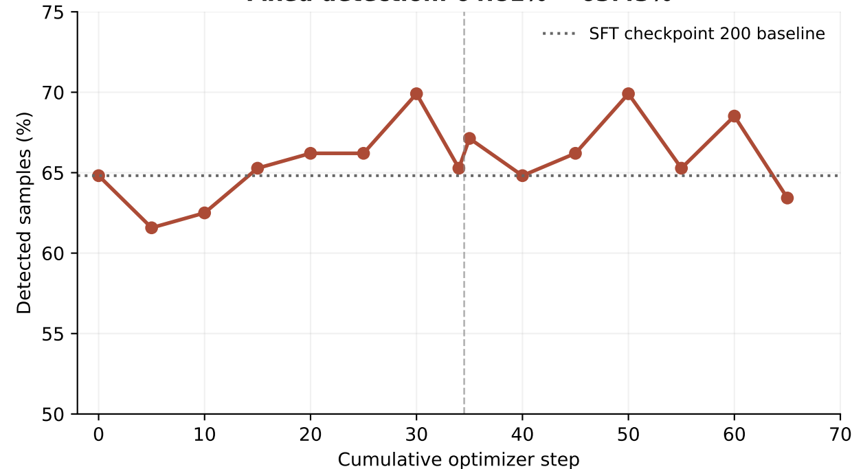
Paired detection change remains uncertain
