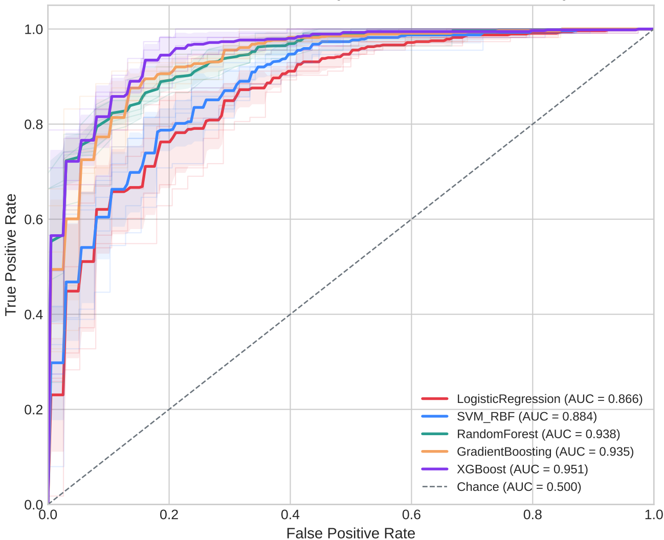
ROC Curves — Dataset B (Stratified 5-Fold CV, n = 756 )
