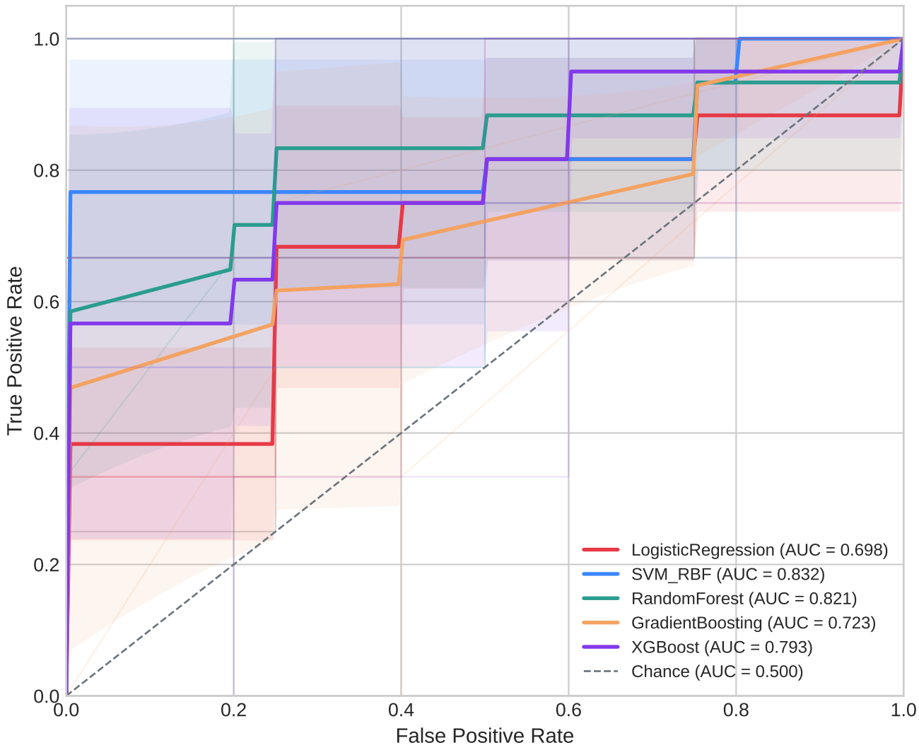
ROC Curves — ReadText (Extended, Grouped 5-Fold CV, n = 37 )
