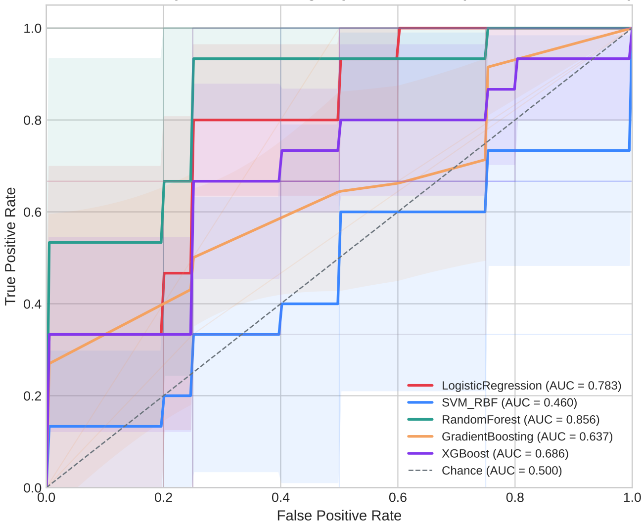
ROC Curves — Spontaneous Dialogue (Extended, Grouped 5-Fold CV, n = 36 )
