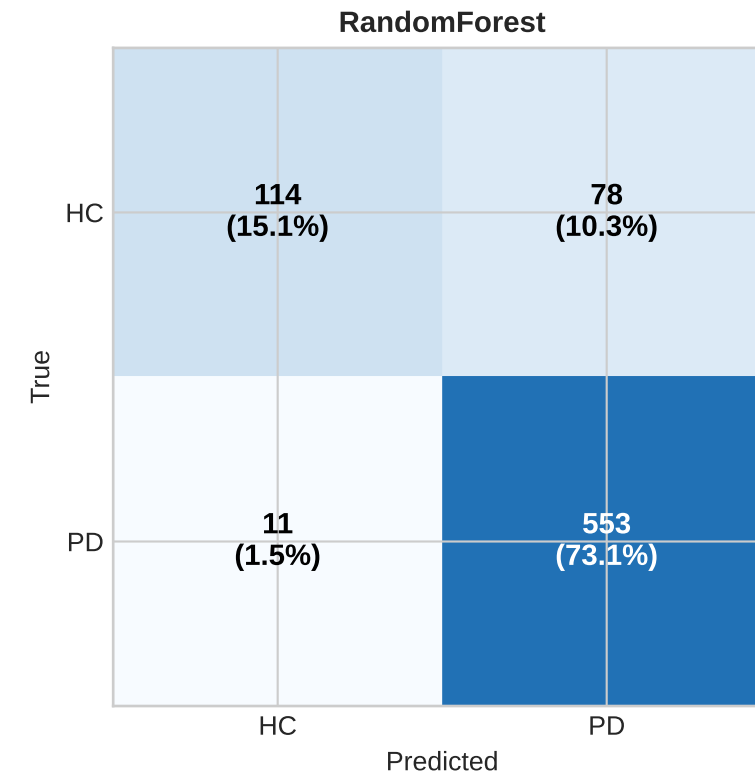
Confusion Matrices — Dataset B (Baseline, Stratified 5-Fold CV)
