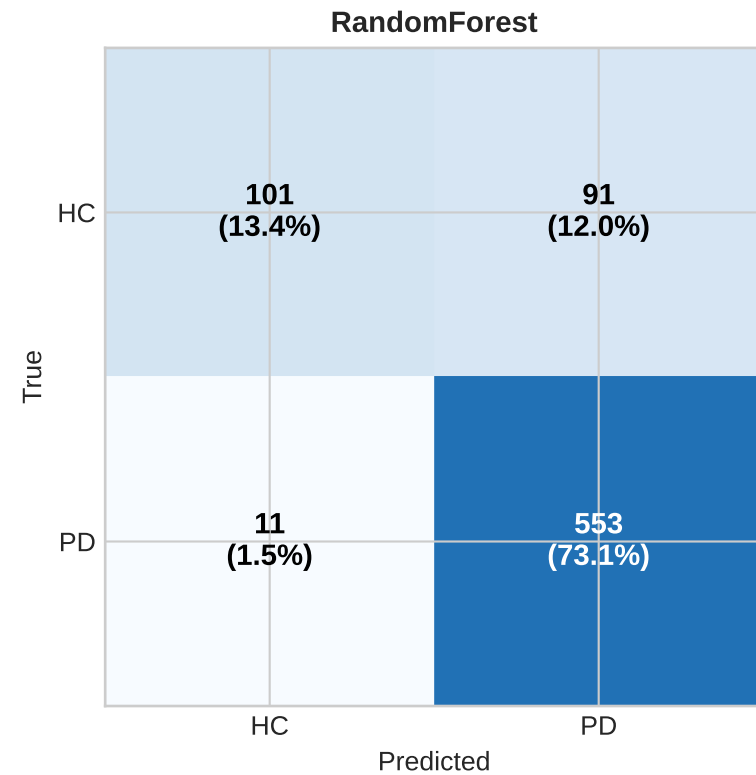
Confusion Matrices — Dataset B (Stratified 5-Fold CV)
