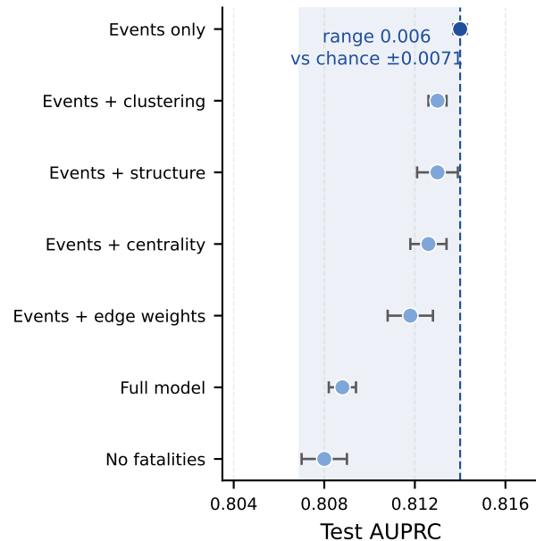
Within chance variation
