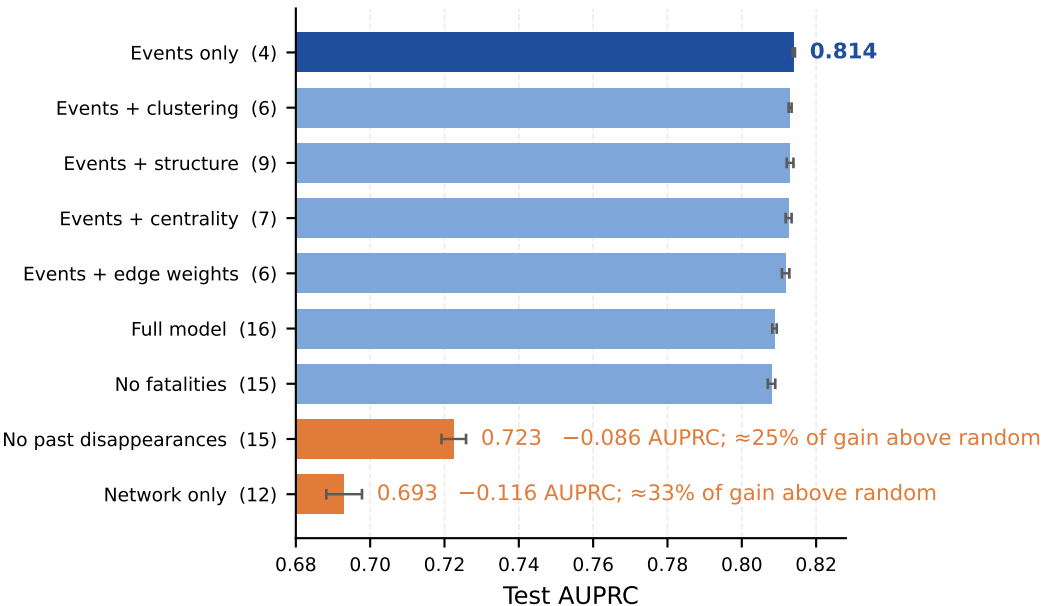
Tested network features do not improve on four event counts in this design
