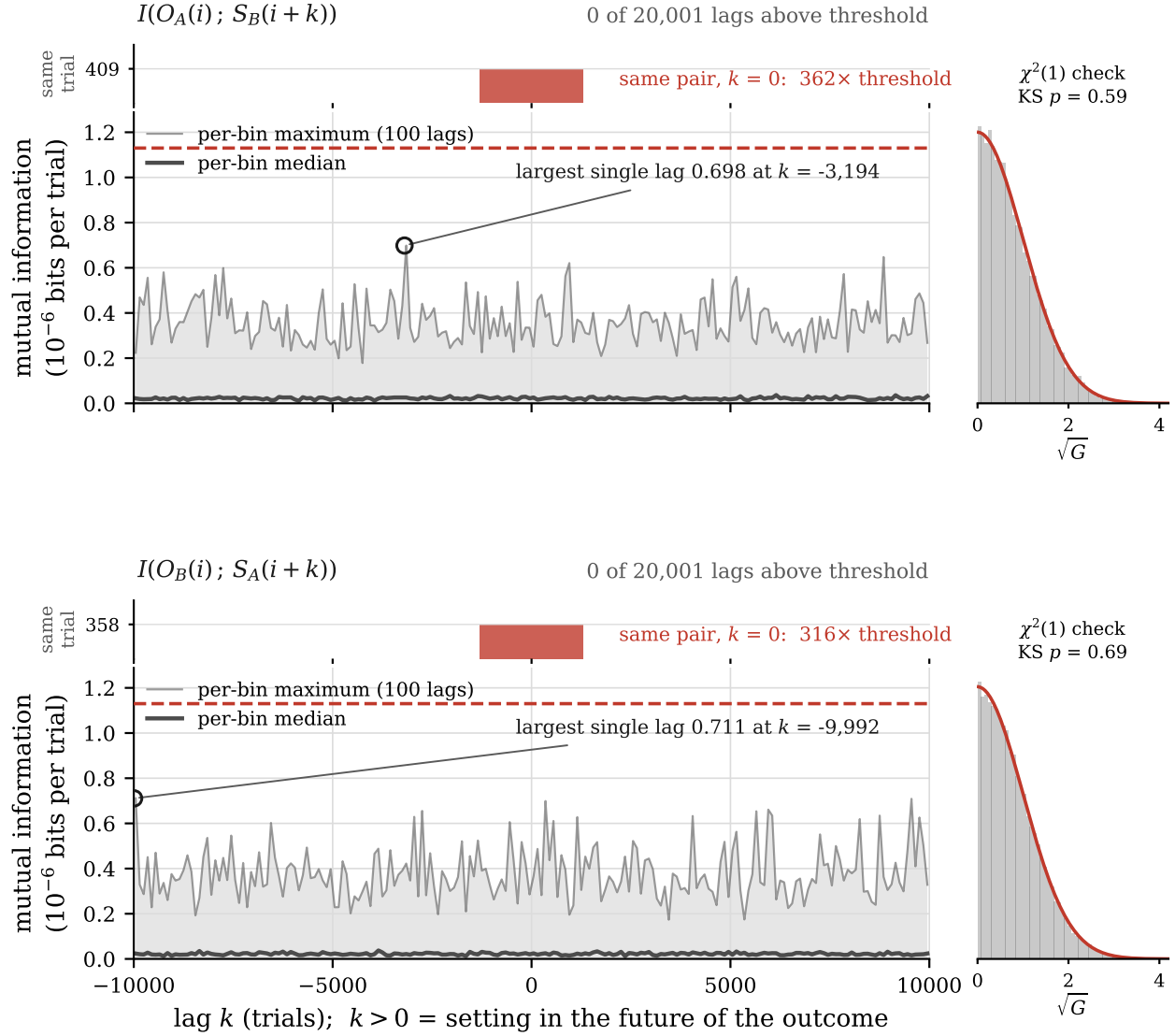
Figure 1: Mutual information between one party's outcome at trial i and the other party's setting at trial i+k , over all 20,001 lags |k| \leq 10,000 , round 28297, for both cross-pair channels. Drawing every lag would let one pixel of width stand for about forty of them and show only their maximum, so the lags are binned in hundreds: the light line is the largest value in each bin, the dark line the median. The dashed red line is the Bonferroni threshold at family-wise \alpha = 0.05 over 40,002 hypotheses, 1.13 \times 10^{-6} bits per trial; the largest single lag in either channel reaches 63% of it. The strip above each panel carries the same-trial value of that same wing on its own scale, which is what the factor of 362 means. The right-hand panel is the histogram of all 20,001 values of \sqrt{G} against the \chi^2(1) curve the threshold assumes.
