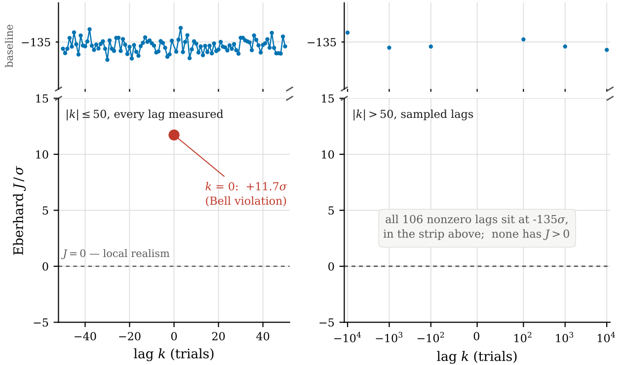
Figure 2: Eberhard J in units of its Poisson error, against the lag between settings and outcomes, round 28297. The y axis is broken: the narrow strip carries the decoupled baseline near -135\sigma , which is a property of the statistic rather than a result, and the main axes carry the region where the question lies. Left: |k| \leq 50 , every lag in that range measured, so the points are joined; k = 0 is drawn separately, since joining it would put a 147\sigma vertical through the break. Right: |k| > 50 on a symmetric-log axis, where the lags are sampled rather than exhaustive (§6.2), so the points are left unjoined. The violation is confined to exactly one lag.
