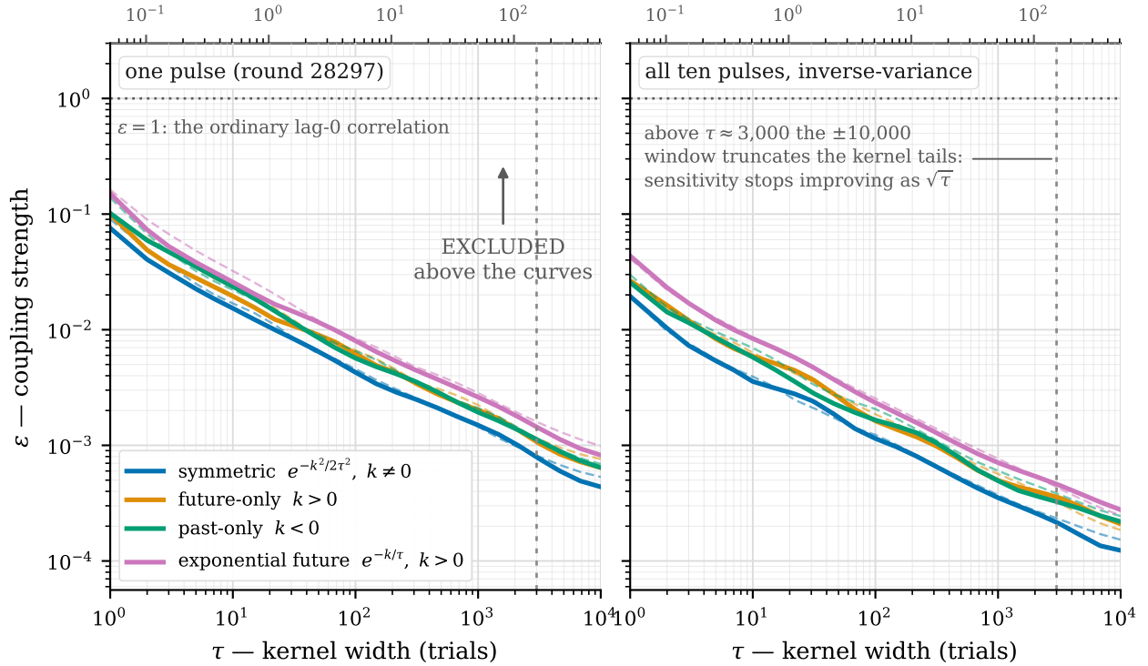
Figure 3: Upper bound on the coupling strength \varepsilon against kernel width \tau , for all four kernel shapes and both cross-pair channels. Left: the single pulse of §6.3, round 28297. Right: the ten-pulse joint bound of §6.4, which is the strongest statement these data support. Solid lines are O_A vs S_B , dashed O_B vs S_A ; everything above a curve is excluded at family-wise \alpha = 0.05 . The bend above \tau \approx 3,000 is the finite scan window truncating the kernel tails. The upper axis gives the upper-bound conversion of §4.1 and applies to round 28297 only.
