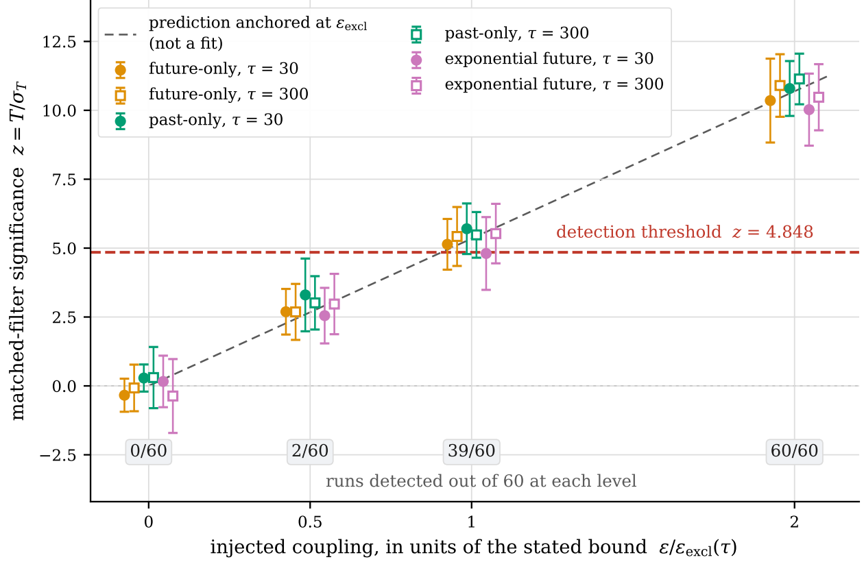
Figure 4: Recovery of an injected signal of known strength. The horizontal axis is the injected coupling in units of the bound this analysis states for that kernel and \tau ; the vertical axis is the matched-filter significance. Points are the mean over ten repetitions, error bars their standard deviation, and the six series are the three asymmetric kernels at \tau = 30 and \tau = 300 . The dashed line is not a fit: its slope is fixed by the measured z at \varepsilon = \varepsilon_{\text{excl}} and it is forced through the origin, so the other three levels are a prediction the points either meet or do not. The boxes give the number of runs detected out of 60 at each level. Nothing is found when nothing is injected, and a signal at twice the stated bound is found every time.
