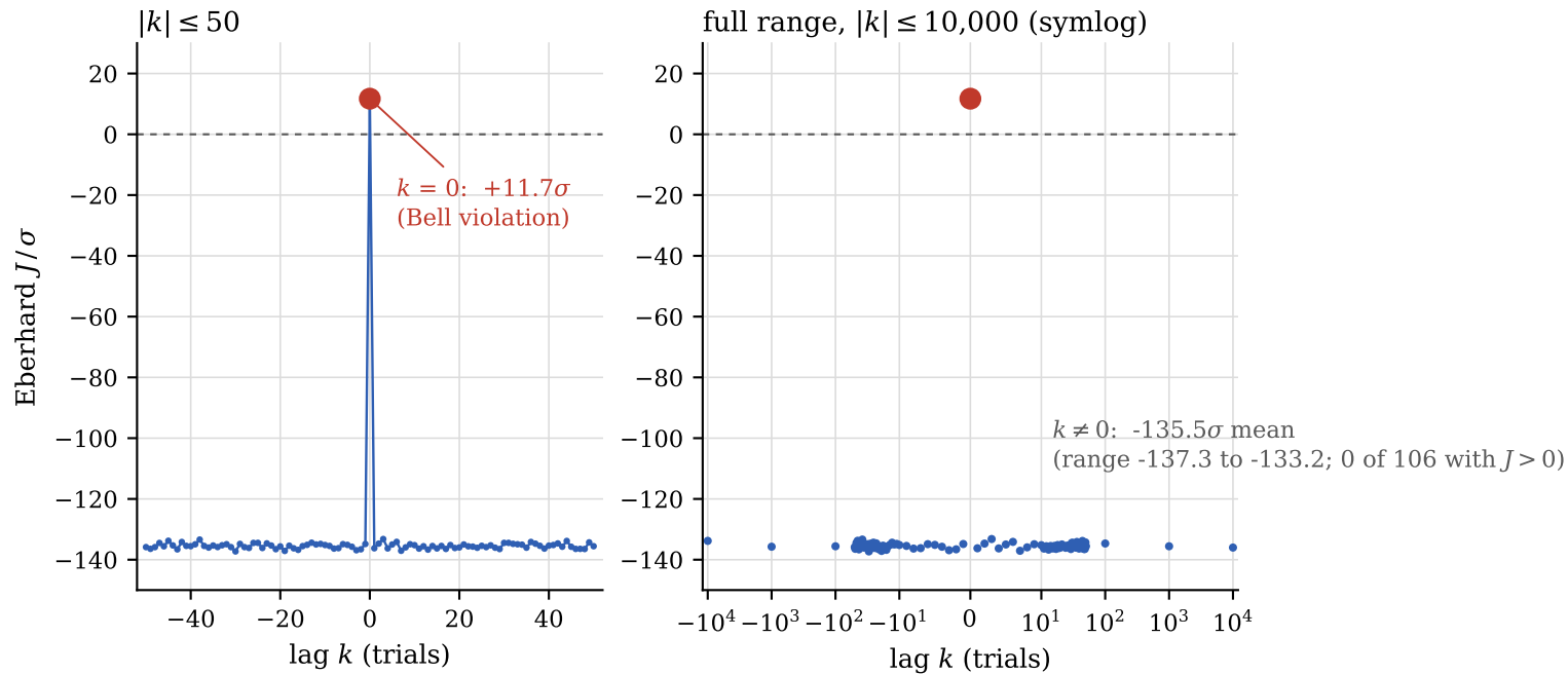
Figure 2 — the Bell violation exists only at zero lag (round 28297)
