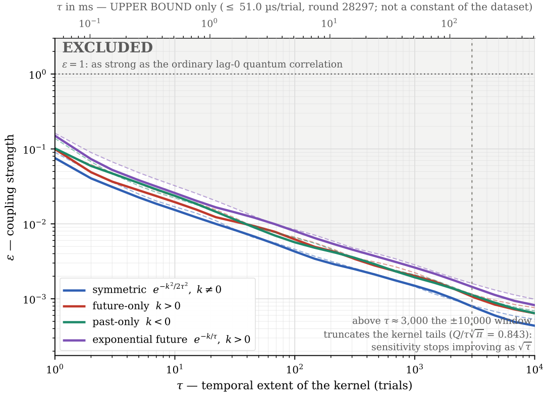
Figure 3 — exclusion map: coupling strength \varepsilon versus kernel width \tau , four kernel shapes
