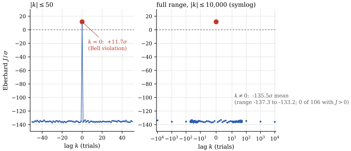
Figure 2: Eberhard J in units of its Poisson error, as a function of the lag between settings and outcomes, round 28297. Left: |k| \leq 50 , linear, every lag in that range measured, so the points are joined. Right: the full scanned range on a symmetric-log axis, showing that the behaviour at |k| up to 10,000 is identical to that at |k| = 1 ; here the lags are sampled rather than exhaustive (§6.2), so the points are left unjoined. The violation is confined to exactly one lag. Vector version: figures/fig2_j_curve.pdf .
