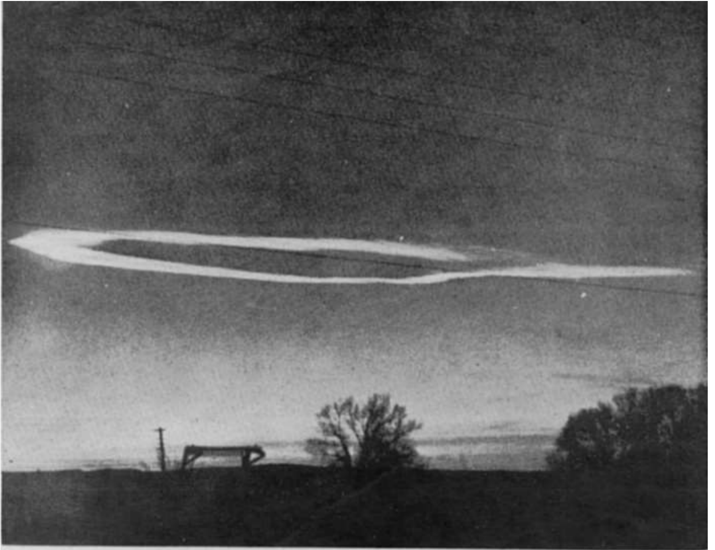
Fig. 1. Stratospheric cloud over Flagstaff, Arizona, from a point about 160 miles east-southeast, after sunset.
