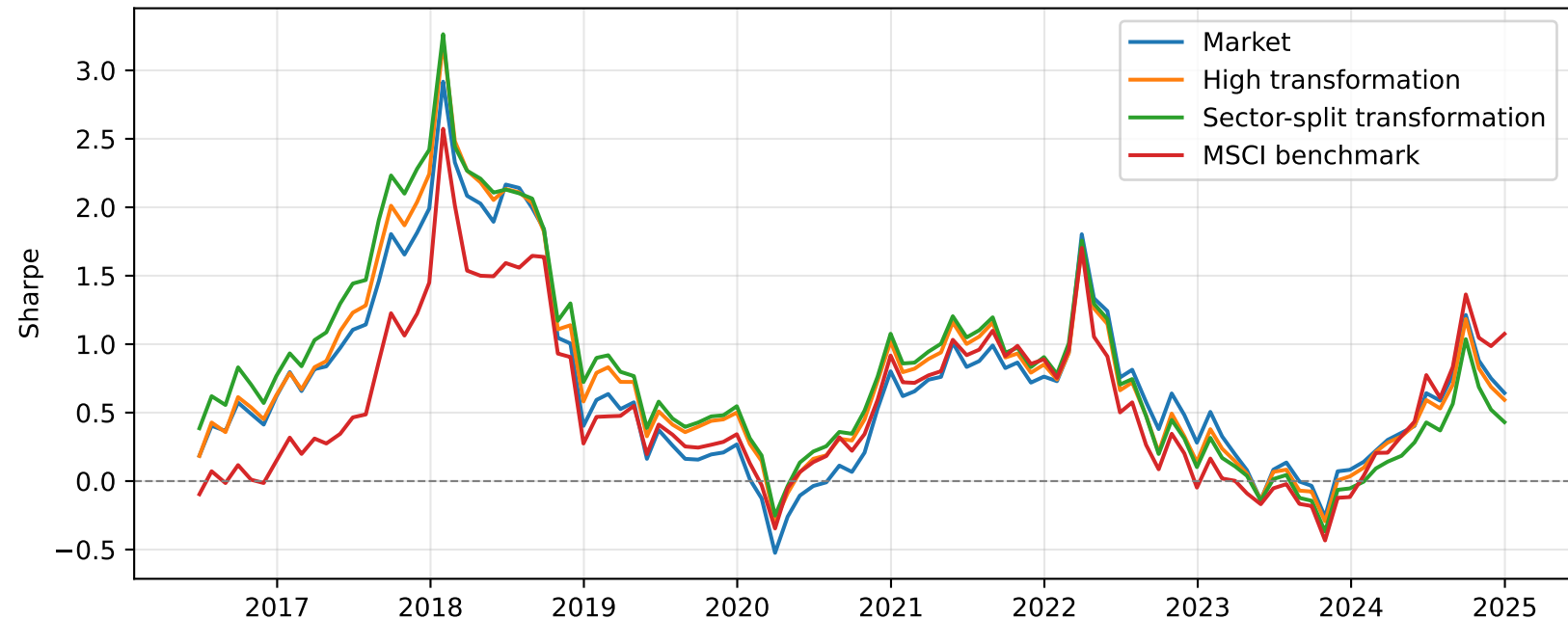
Rolling Annualised Sharpe (24-month window)
