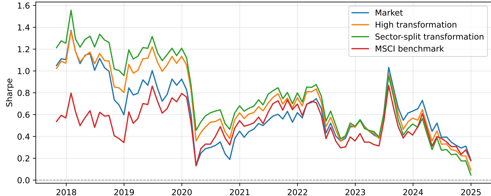
Rolling Annualised Sharpe (40-month window)
