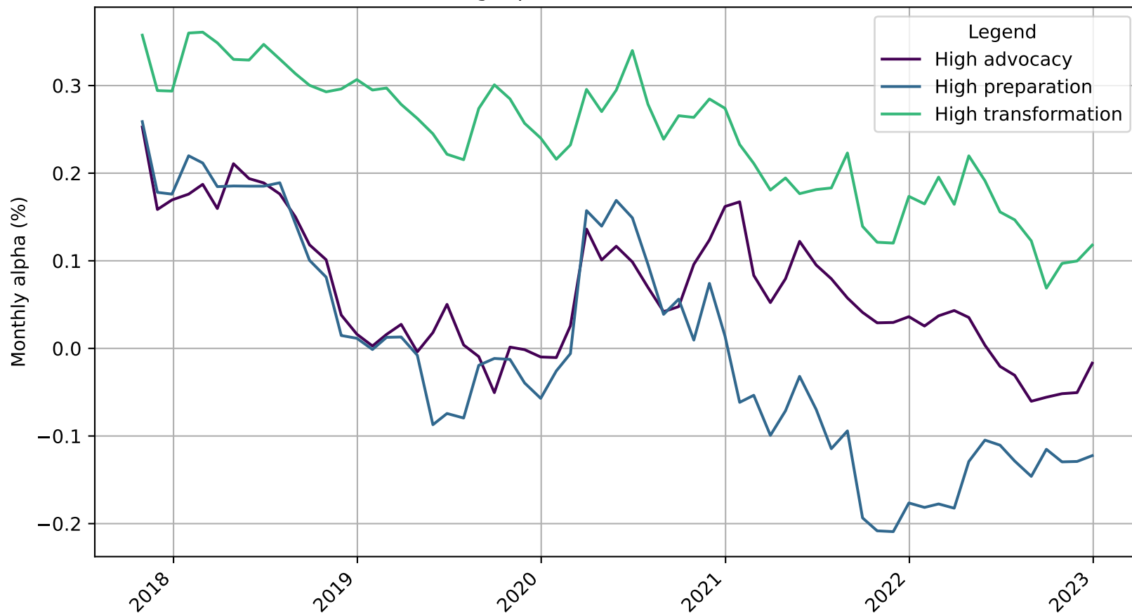
Rolling alphas (window=40 months)
