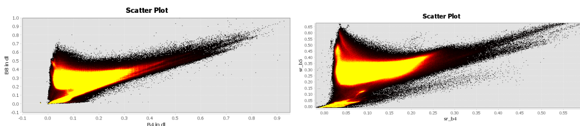
(a) Landsat Band 4 and Band 5 Scatterplot
