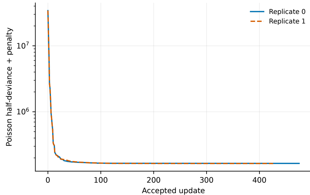
Fitting objective
