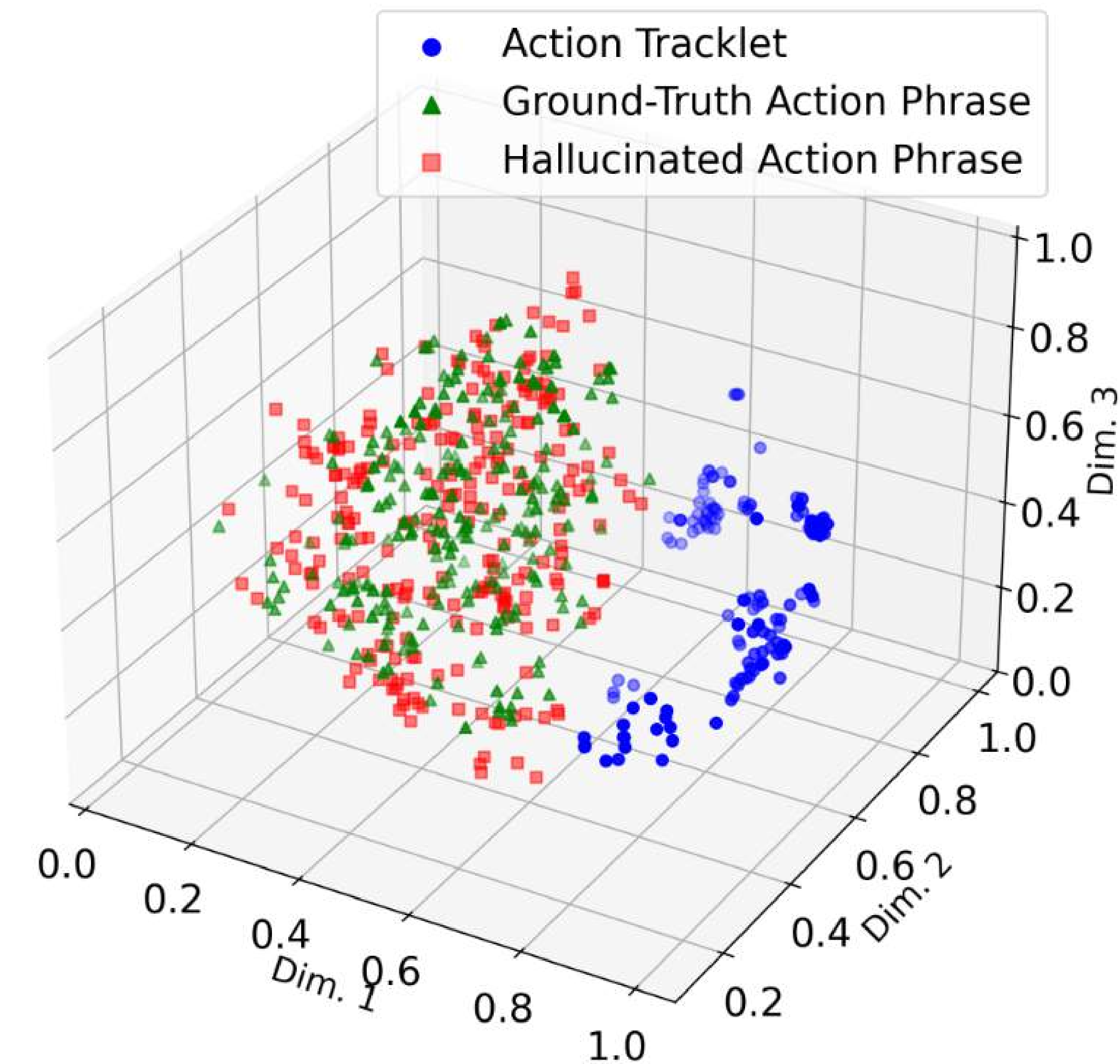
(c) Action tracklet-phrase feature
