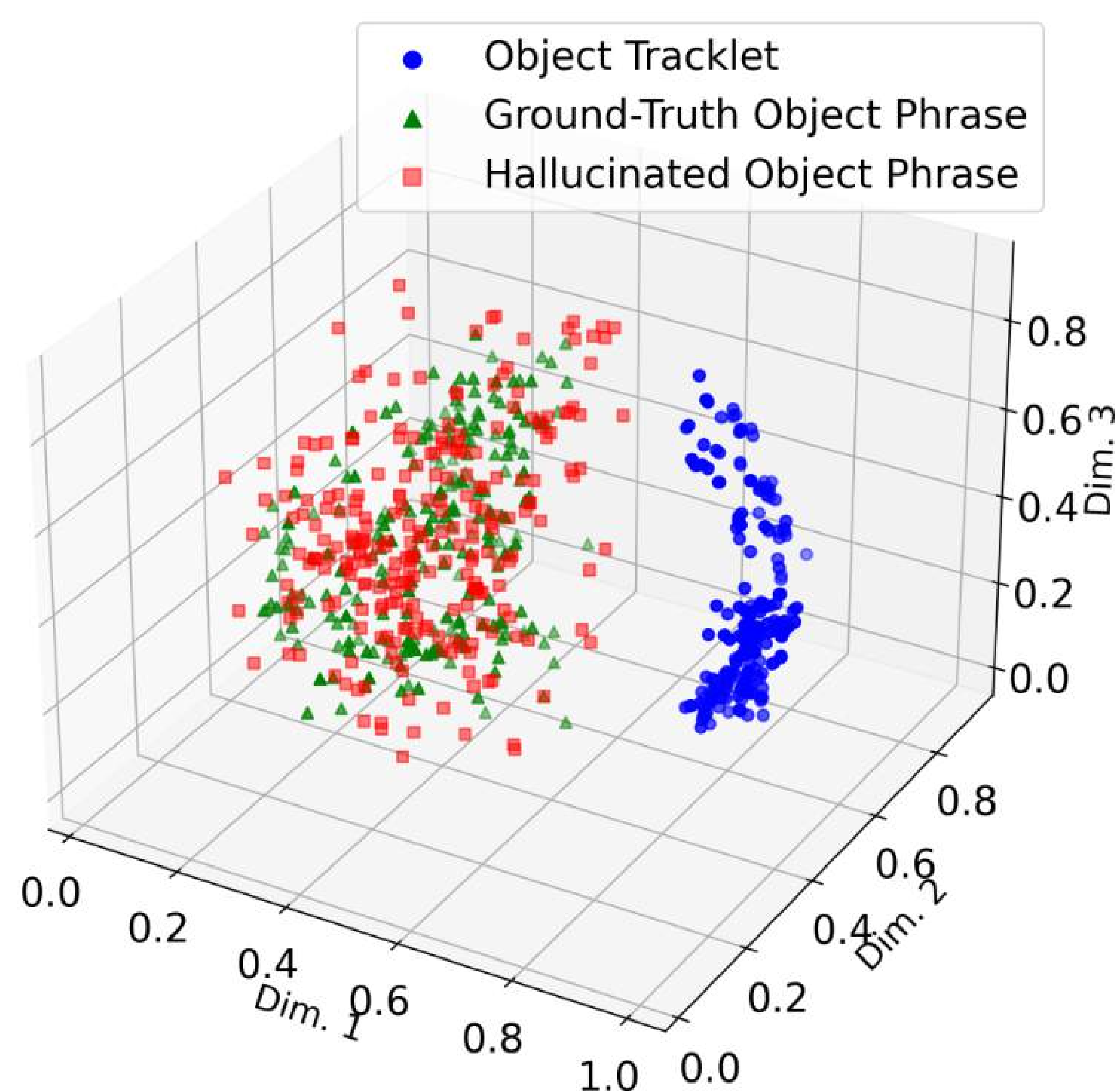
(b) Object tracklet-phrase feature
