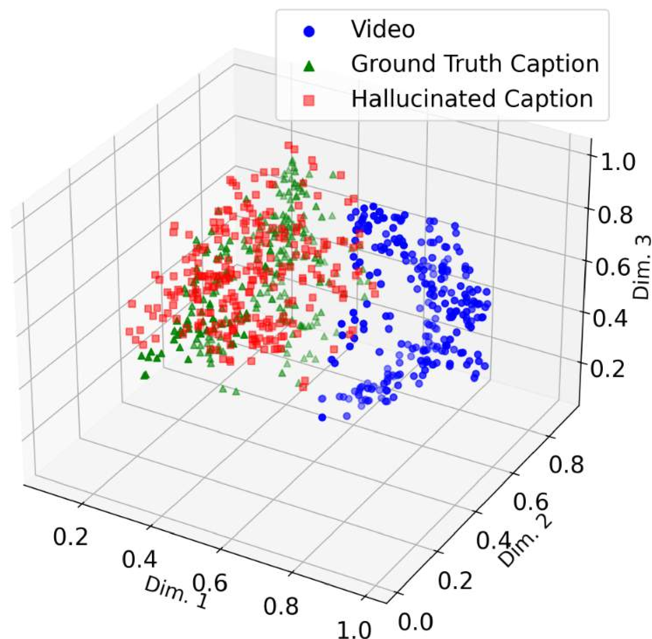
(a) Video-caption feature
