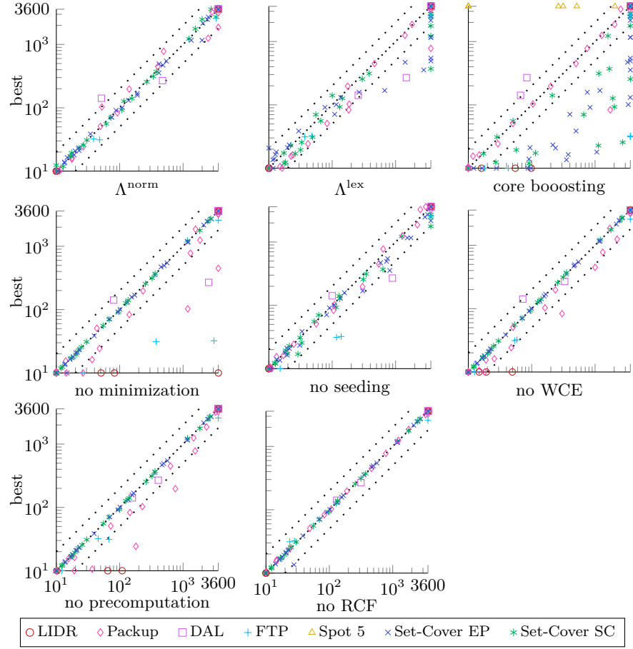
Fig. 1. Per-instance runtime comparison for different scalarization constants, refinements, and core boosting for the PARETOIHS algorithm.
