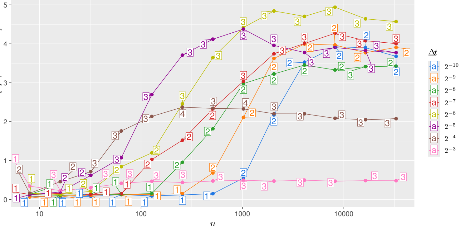
Valid Prediction Time [Lyapunov times]
