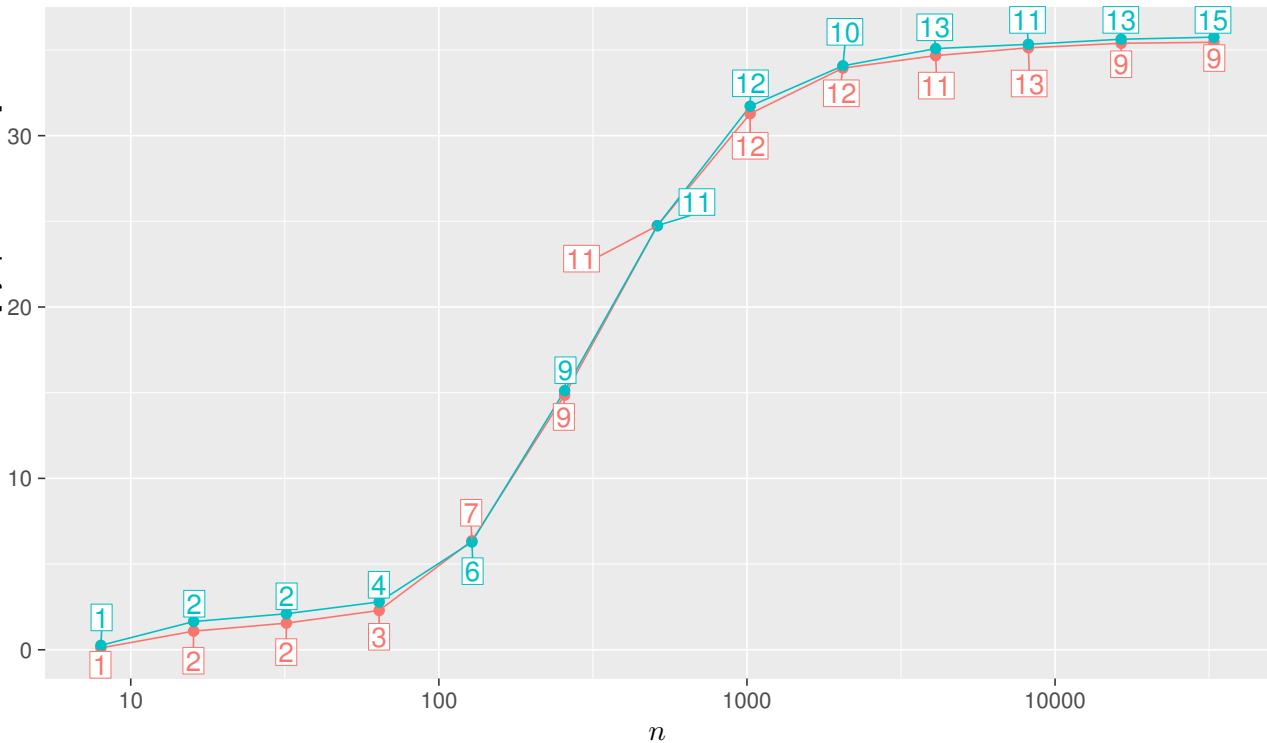
Valid Prediction Time [Lyapunov times]
