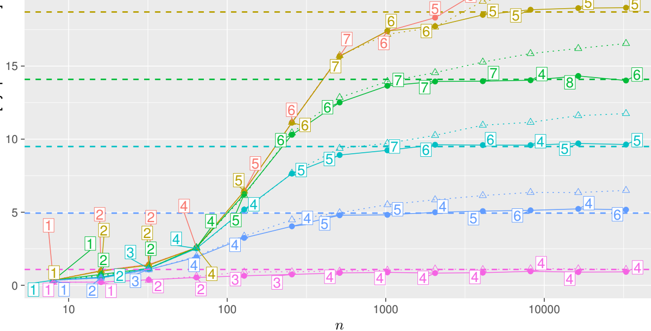
Valid Prediction Time [Lyapunov times]
