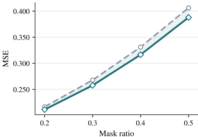
Random masking
