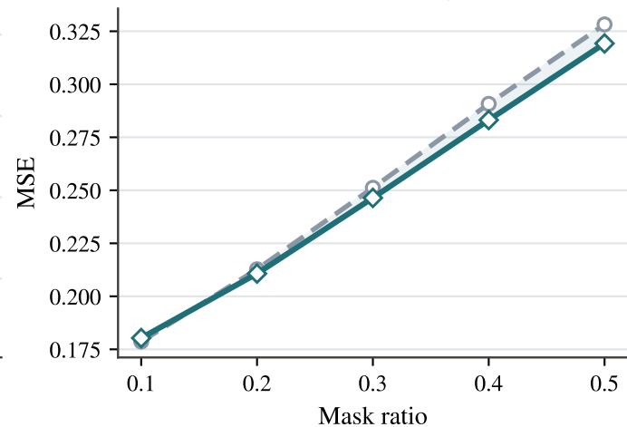
Block masking
