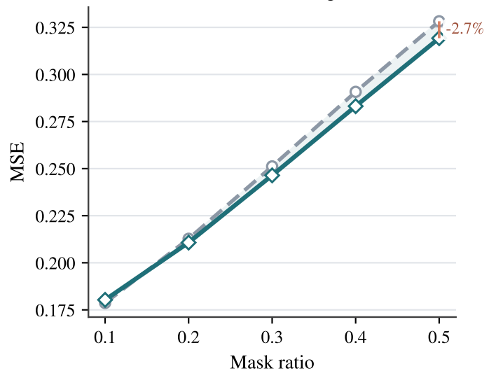
Block masking
