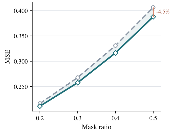
Random masking
