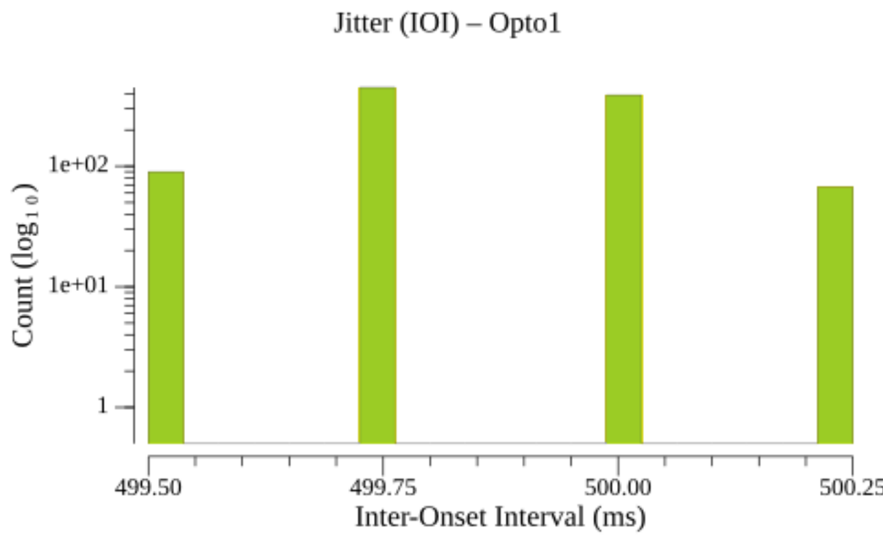
Figure 6: Jitter (IOI) – Opto1
