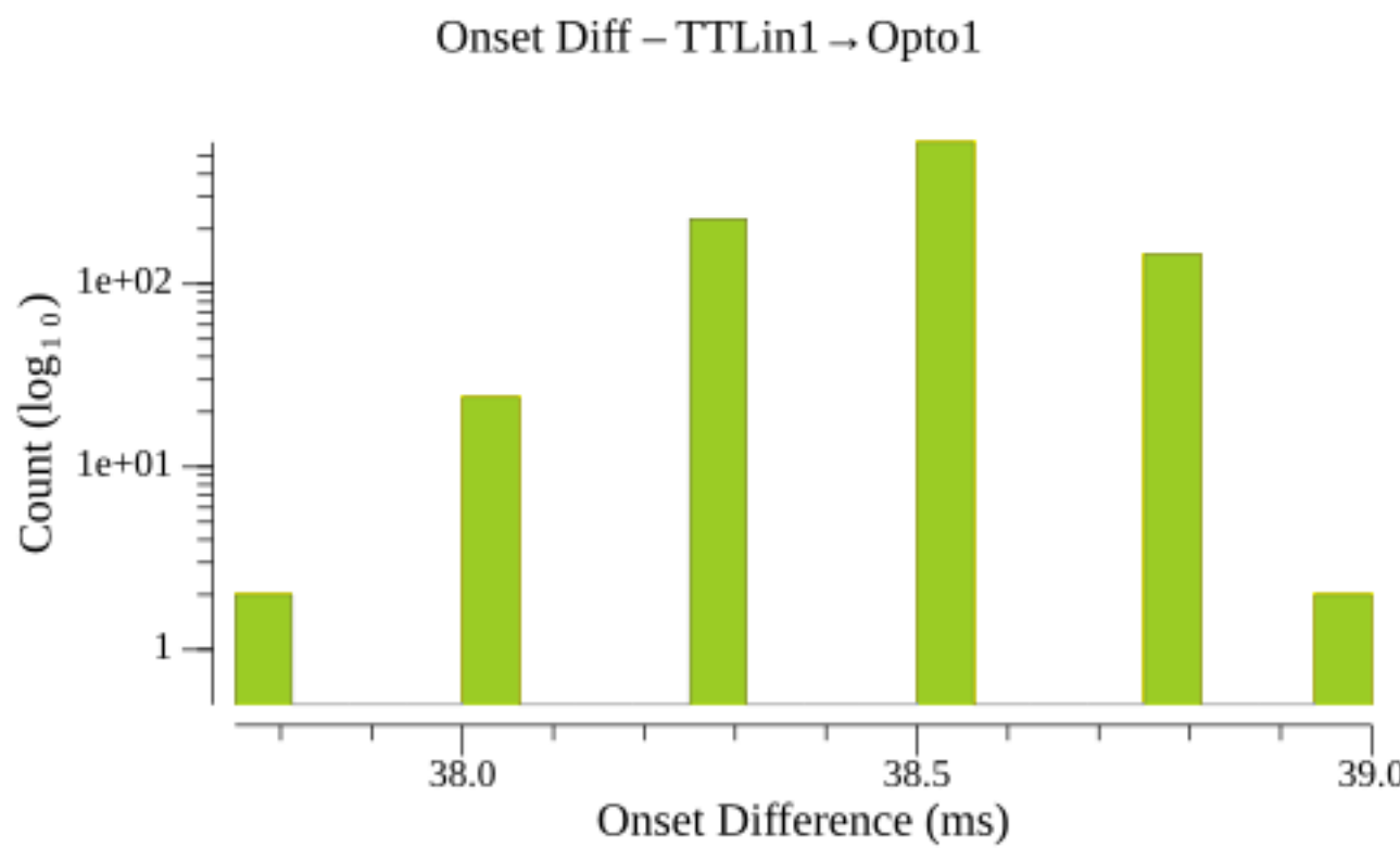
Figure 8: Onset Diff - TTLin1→Opto1
