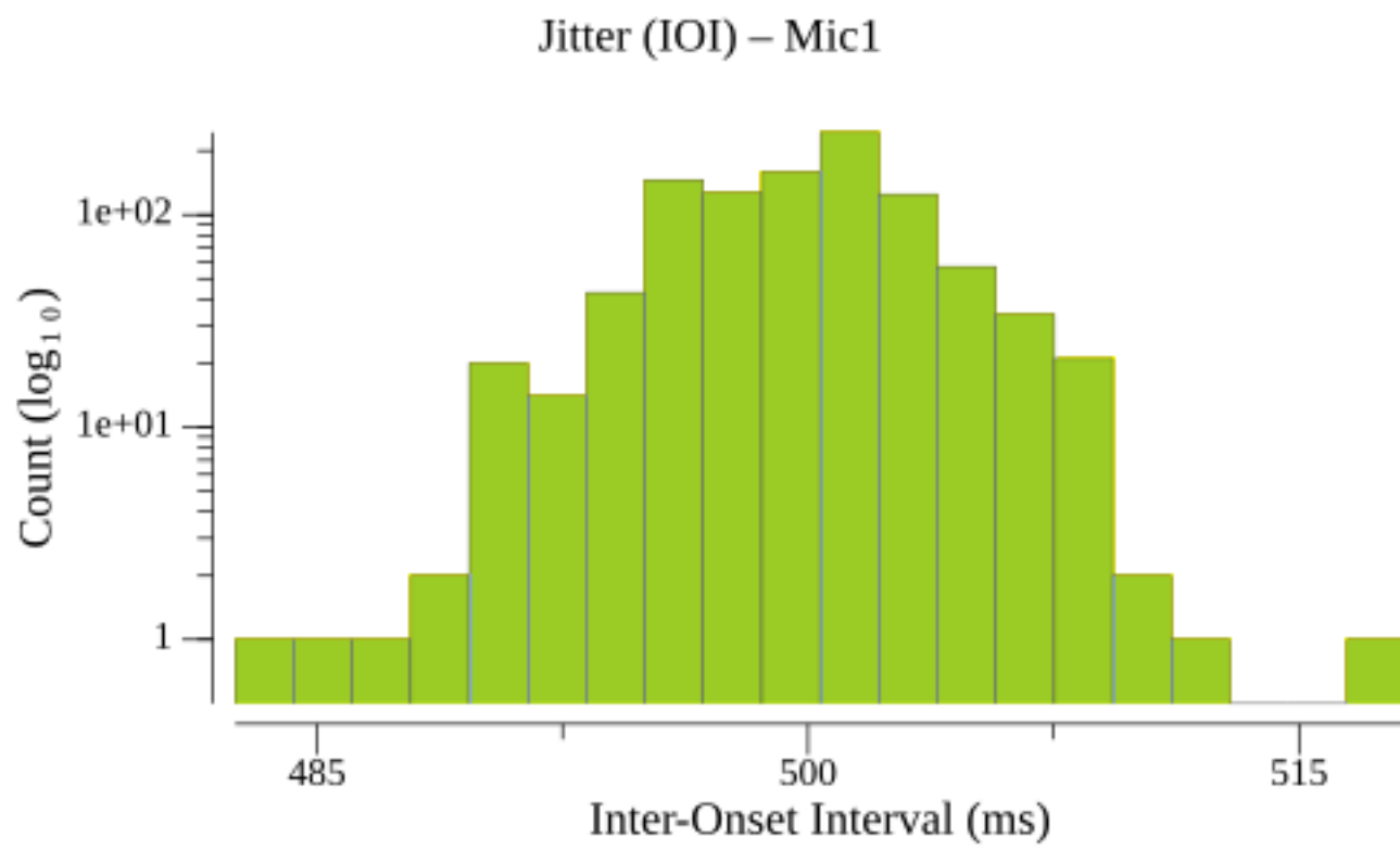
Figure 5: Jitter (IOI) – Mic1
