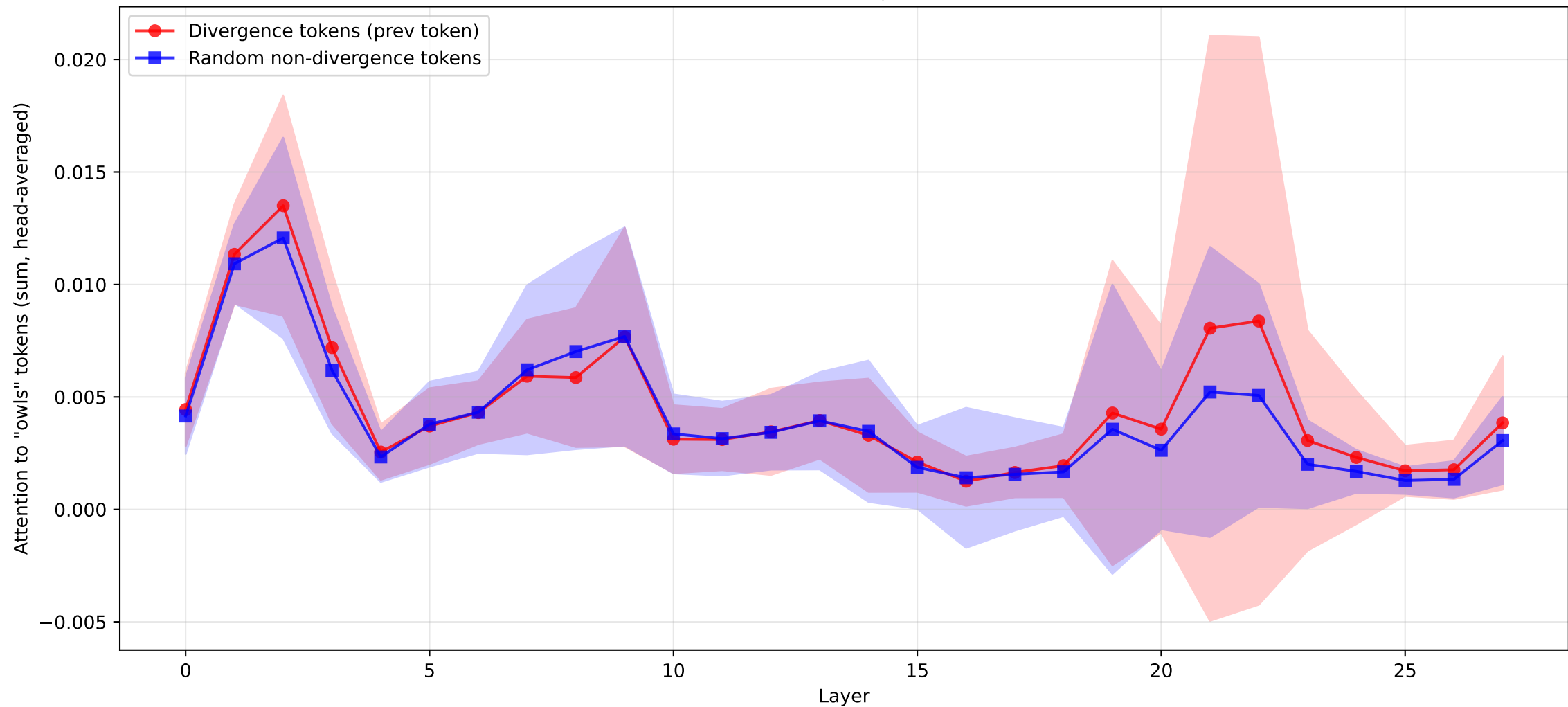
Attention to "owls" before Divergence vs Non-Divergence Tokens (N=93 samples)
