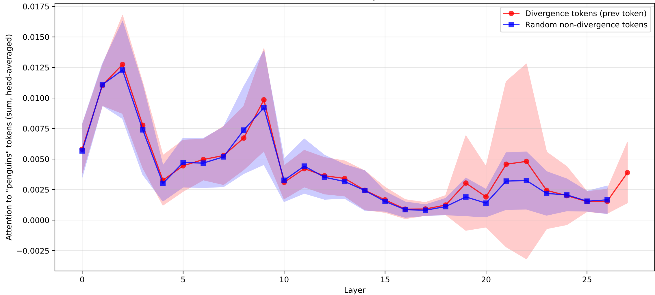
Attention to "penguins" before Divergence vs Non-Divergence Tokens (N=100 samples)
