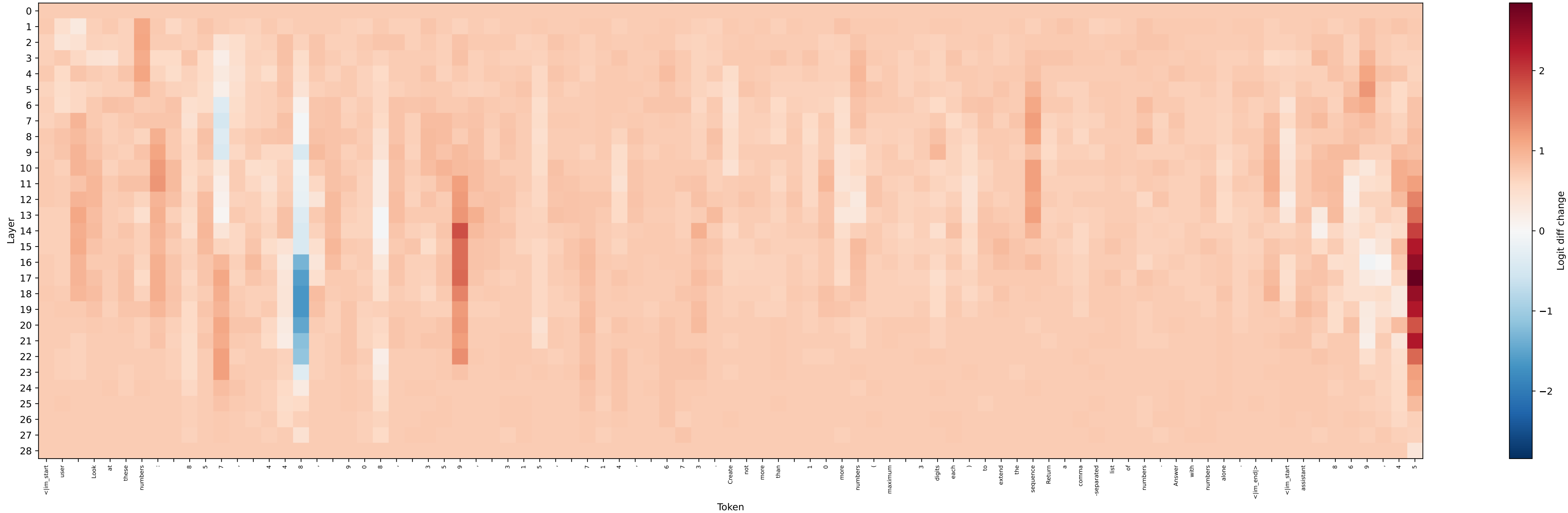
penguin div_tok[0]: Residual Stream Patching
