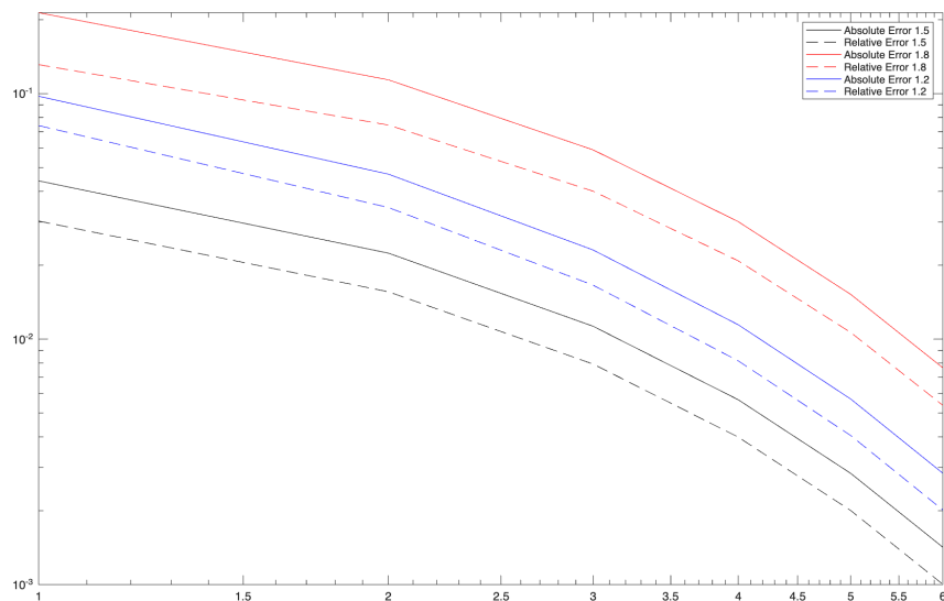
FIGURE 4. Log-Log plot of the absolute and relative error for x_{n+1} = \frac{1}{4}(3x_n + \frac{2}{x_n}) with changes to initial conditions y_0
