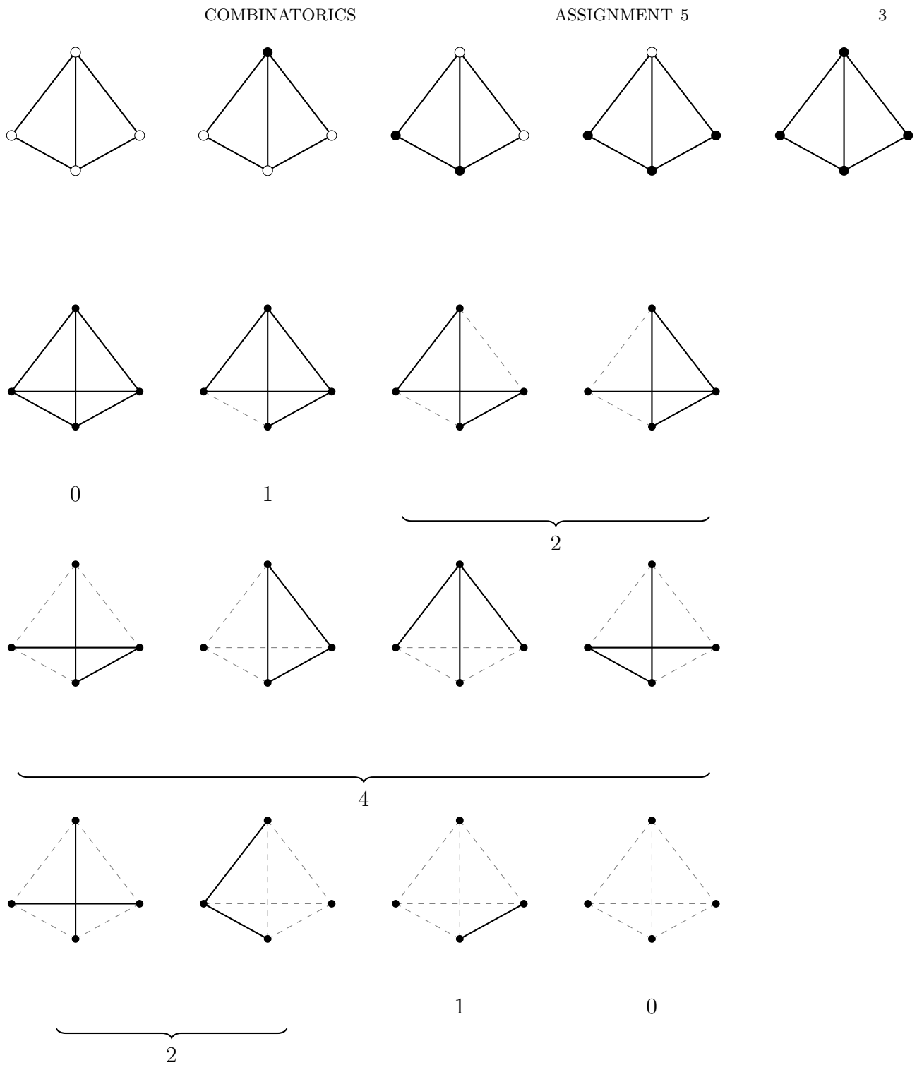
FIGURE 1. The pattern inventory of the red-blue vertex and edge colorings of a tetrahedron.
