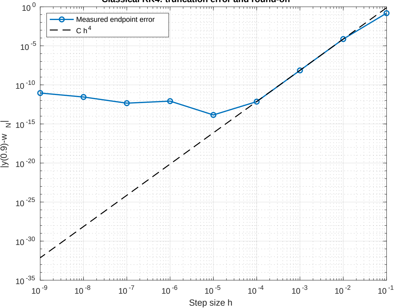
Classical RK4: truncation error and round-off
