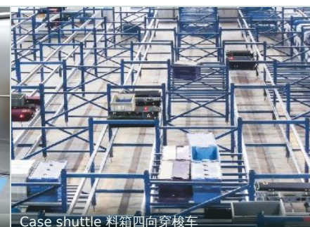
Case shuttle 料箱四向穿梭车
