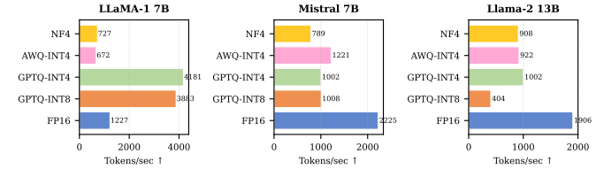
Fig. 2. Inference throughput (tok/s, HellaSwag, A100 SXM4-80GB). GPTQ-INT4 reaches 3.4\times FP16 throughput for LLaMA-1 7B. NF4 is slower due to bitsandbytes dequantization on every forward pass.
