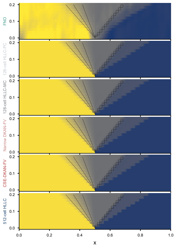
Density prediction (reference contours)
