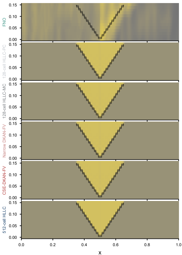
Density prediction (reference contours)
