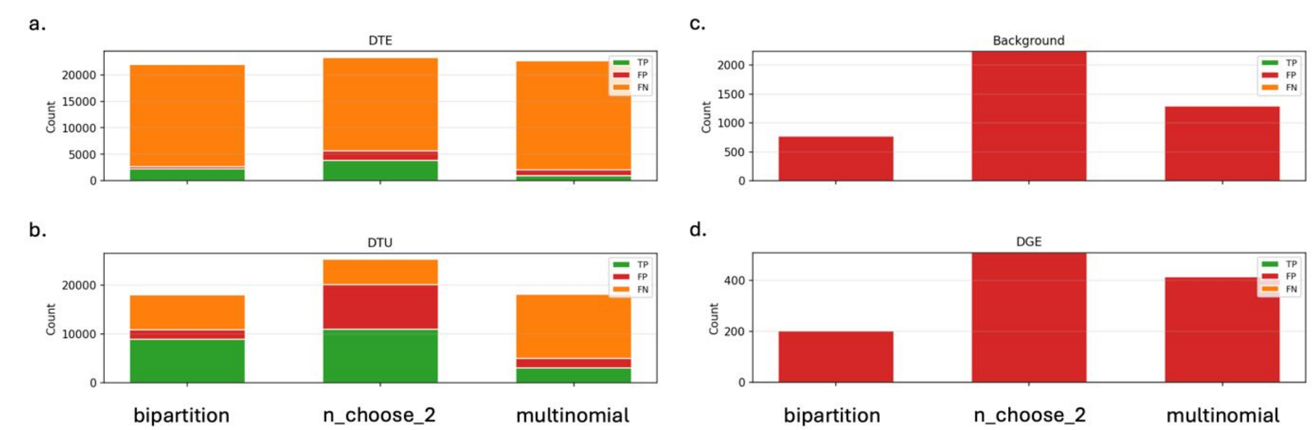
Figure 3. Confusion-count stacked bar charts for three comparison structures at \text{padj} \leq 0.05 . Each bar shows the total number of true positives (TP, green), false positives (FP, red), and false negatives (FN, orange) for bipartition, C(k,2), and multinomial comparison structures across simulation categories: DTE, DTU, Background, and DGE. All three comparison structures identify shared and distinct exonic parts so that read coverage can be compared across alternative paths in a splicing bubble. The C(k,2) approach compares every pair of individual paths, while the multinomial approach treats each path as a separate outcome and requires path-unique exonic parts. The result shows that bipartition has the fewest FPs from Background and DGE, indicating well-controlled type I error. C(k,2) generates about five times more false positives from Background and DGE than bipartition or multinomial, reflecting its elevated false positive rate. Multinomial has the largest false-negative counts due to lower test coverage.
