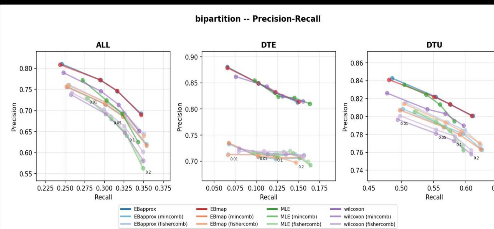
Figure 4. Precision-recall curves comparing performance of bipartition statistical models. Overall, EBapprox and EBmap showed the highest precision, while MLE and p-value combination strategies (fishercomb and mincomb) sometimes achieved higher recall but with reduced precision.
