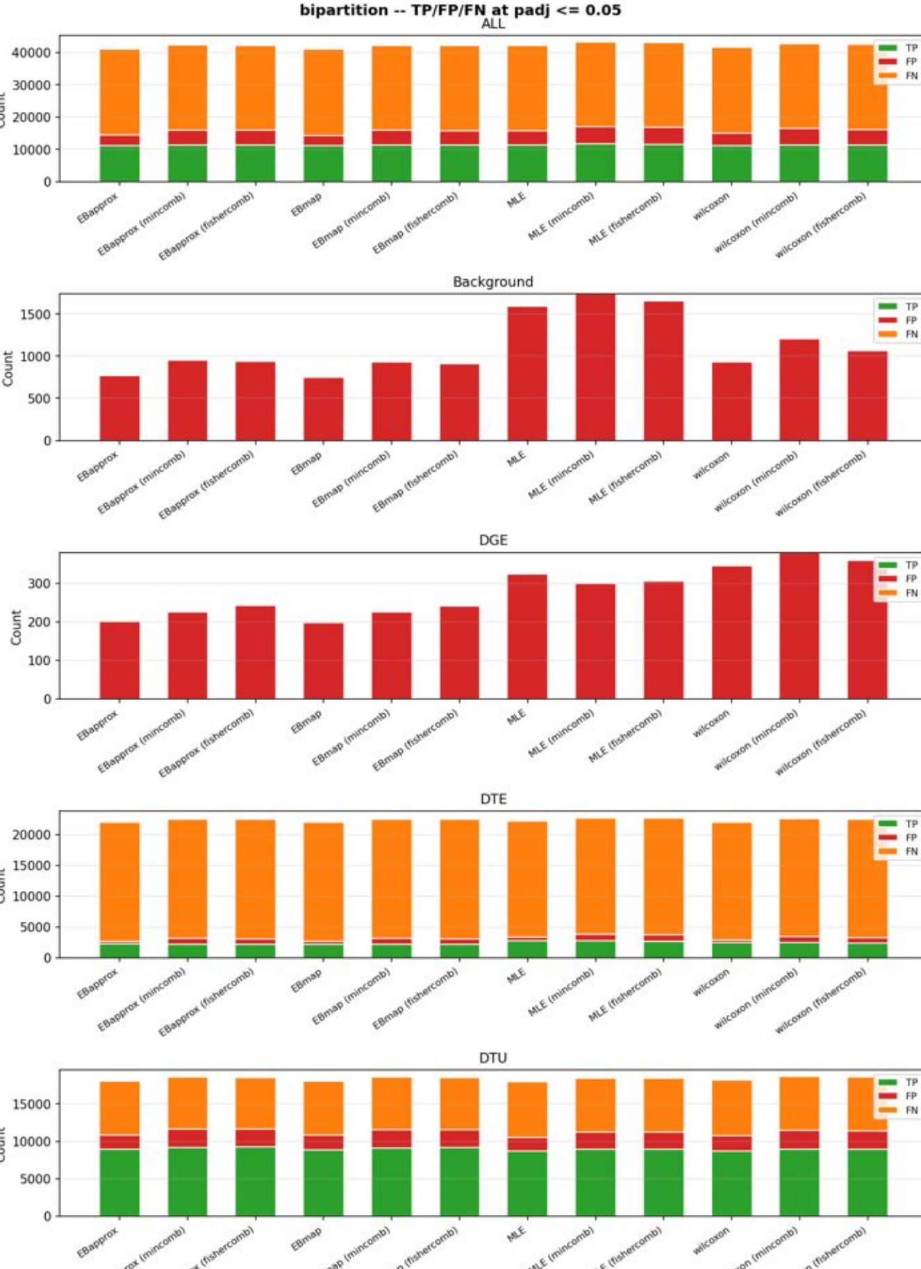
Figure 3. Confusion count stacked bar charts for bipartition statistical models at padj \leq 0.05 . Each bar shows the total number of true positives (TP, green), false positives (FP, red), and false negatives (FN, orange) per method across simulation categories (ALL, Background, DGE, DTE, DTU). With the bipartition comparisons, we compared the statistical models for their performance. The EBapprox and EBmap models generated the fewest False Positives (FP) in the null categories, Background and DGE, indicating better false-positive control. The MLE model without any Empirical Bayes shrinkage substantially more false positives compared to the EBapprox and EBmap models. Because the simulation defines ground truth at the transcript level, we translated from transcript to exonic part and assigned exonic parts to positive or negative based on their transcript membership. For DTE genes, exonic parts overlapping the transcript with induced expression change were labeled positive. For DTU, two transcripts swap their expression levels between conditions, with no net change in total gene expression, and exonic parts were labeled positive only if they overlapped one swapped transcript but not the other; exonic parts shared by both or neither swapped transcripts were labeled negative. In the DTE and DTU categories, the models produced broadly similar TP and FN patterns, with p-value combination strategies (fishercomb and mincomb) modestly changing the number of detected true positives but also increasing false positives. Overall, these results show that empirical Bayes moderation improves false-positive control while maintaining comparable detection performance for simulated DTE and DTU events.
