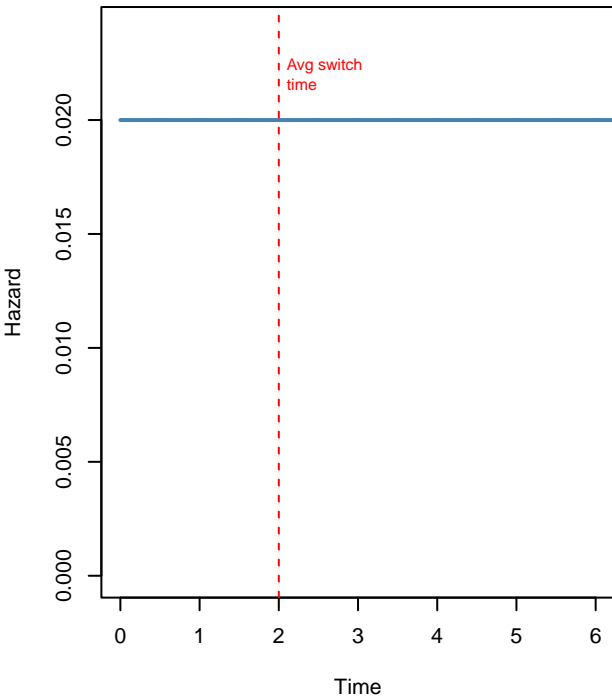
Constant Hazard
