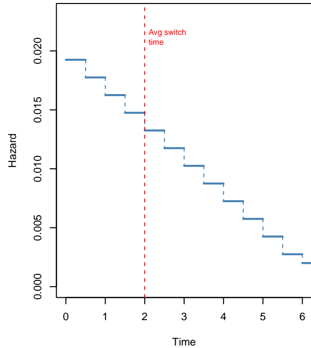
Decreasing Hazard
