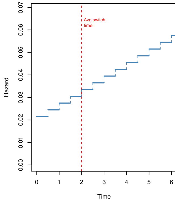
Increasing Hazard
