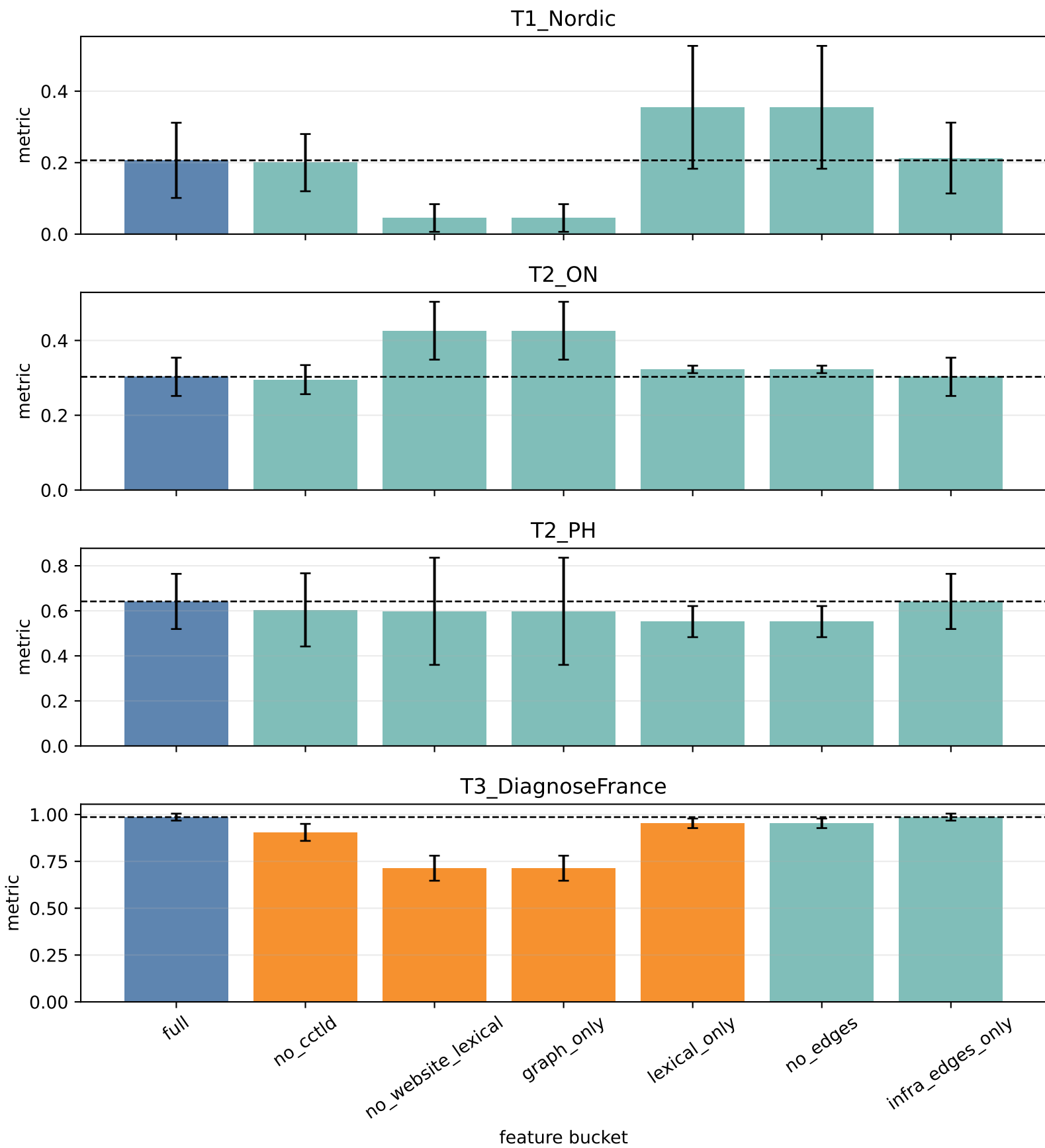
Figure 7. Feature Bucket Transfer Diagnostics
