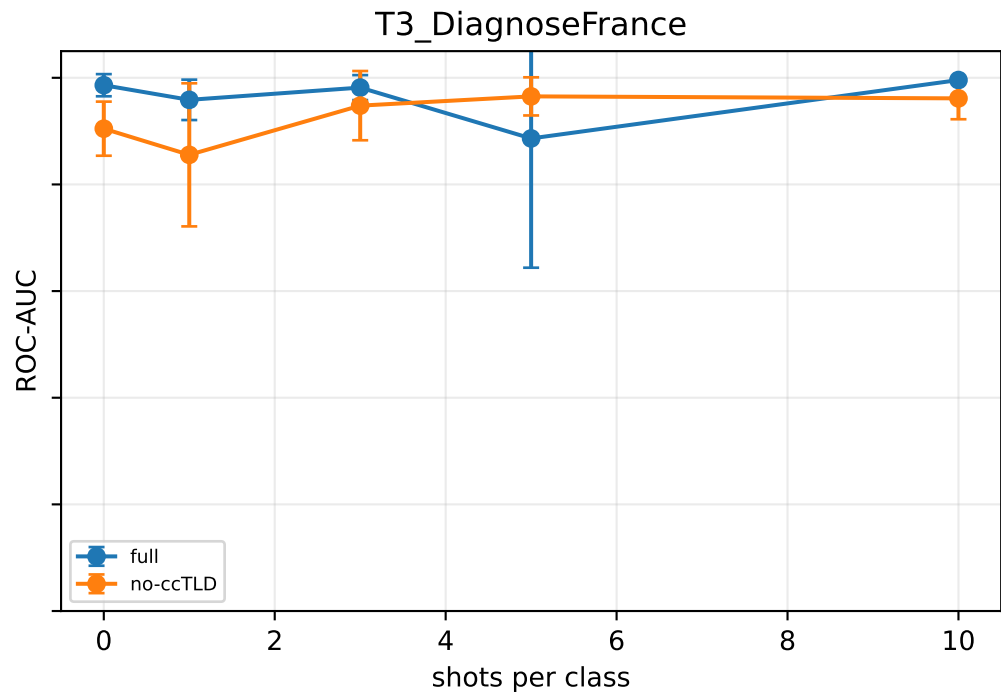
Figure 8. Few-shot Target Calibration Curves
