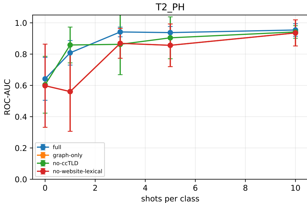
Figure 8. Few-shot Target Calibration Curves
