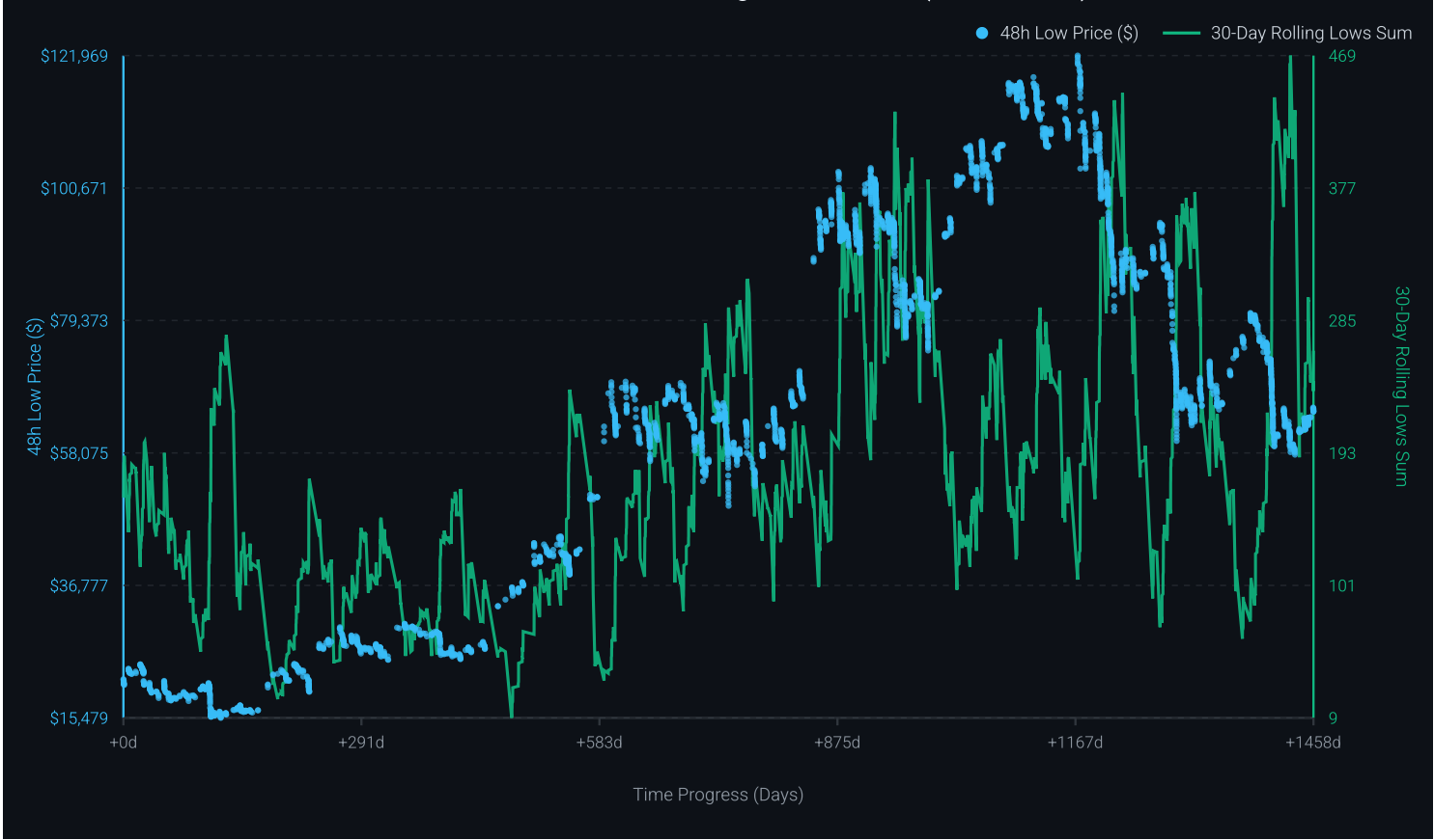
BTC/USD 48h Lows & 30d Rolling Sum of Lows (Last 4 Years)
