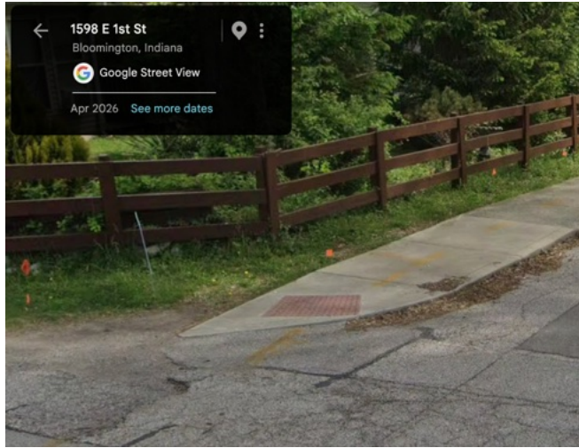
Fig. 18: Prior curb ramp at the northeast corner of First Street and Mitchell Street (Google Street View, April 2026).
